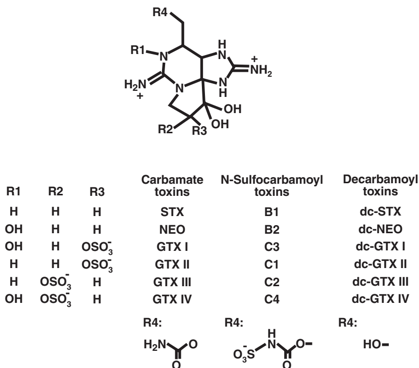
Fig. 17. Structure of PSP-toxin. STX is saxitoxin (redrawn from Sullivan 1993).
