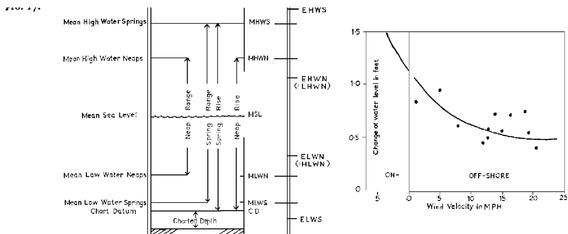
Figure 1. (A) Left - The nomenclature of tidal levels for mean springs and neaps, showing the extent of the range and the rise as related to 'Chart Datum'. Extreme levels for springs and neaps are shown in the separate column. (B) Right - The effect of onshore and offshore winds in raising and lowering the water level of predicted tides.
