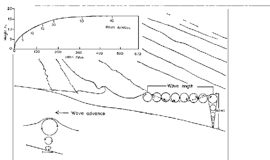
Figure 3. Marine Waves. Orbits shown at intervals in the propagation of a wave with the simultaneous position of water particles and the profile of the water surface.
