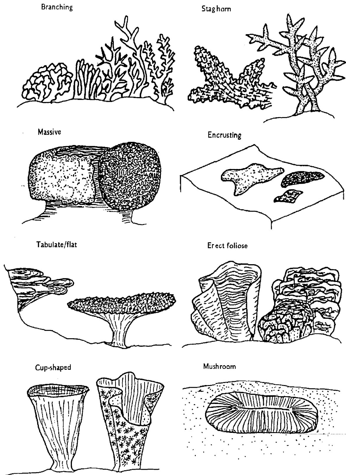
Figure 9. Various morphological types of hard coral and how they could be described in a survey transect.
