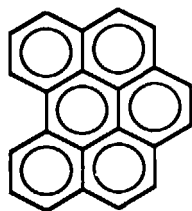
Benzo[ghi]perylene 191-24-2
