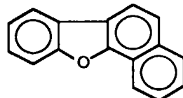
Benzo[b]naphtho- [2,1-d]furan 239-30-5
