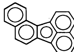
Benzo[j]fluor- anthene 205-82-3
