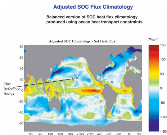
Global estimates of the annual mean net heat input to the oceans from in situ measurements. [Courtesy S. Josey, National Oceanography Centre, Southampton]
