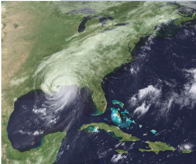
Hurricane Katrina 2005. WCRP research will help to determine if hurricanes and other extreme weather events will become more frequent or intense in the future. [Earth Observatory/NASA]
