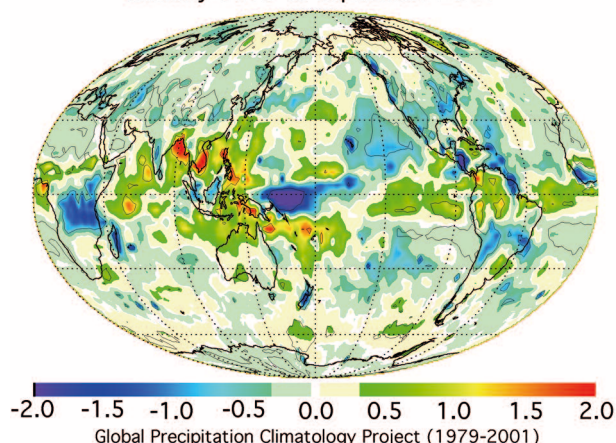
23 Year Change in Global Precipitation Anomalies January 1979 to September 2001
