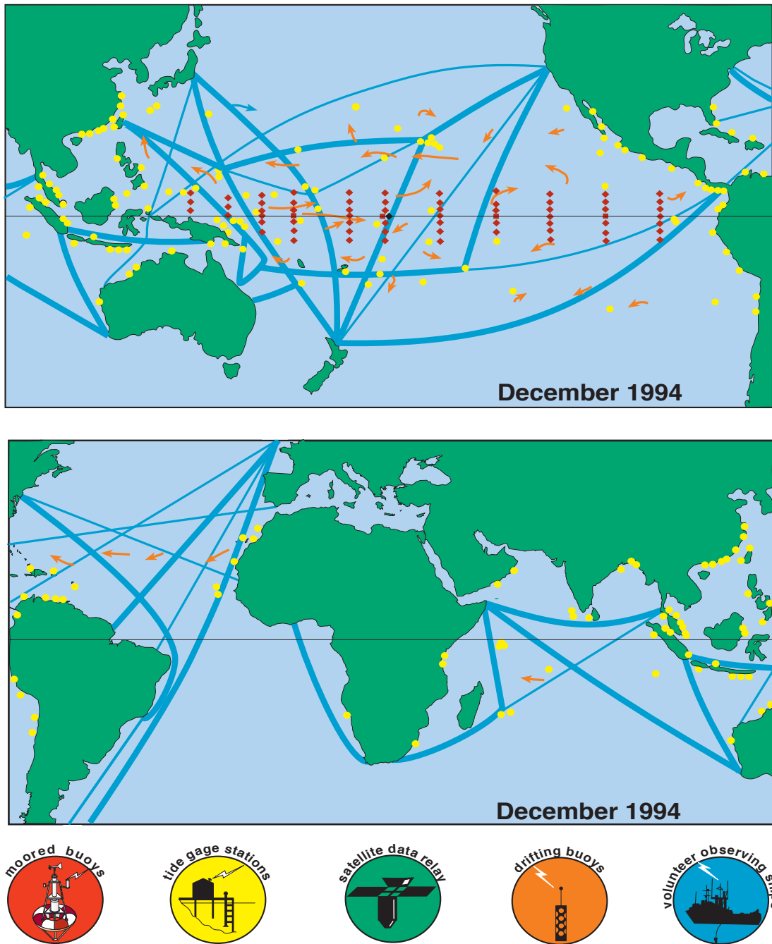
Figure 2. The in situ TOGA observing system in December 1994: (a) Pacific Ocean; (b) Atlantic and Indian Oceans. Symbols as for Figure 1 (from McPhaden et al., 1998).
