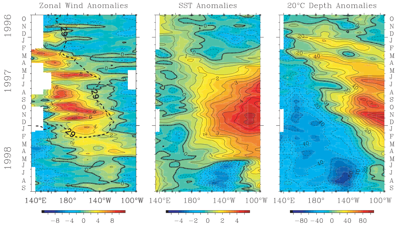
Figure 13. Anomalies in surface zonal wind (in \text{m}\cdot\text{s}^{-1} , left), sea surface temperature (in ^{\circ}\text{C} , middle), and 20°C isotherm depth (in m, right) from October 1996 to September 1998. Analyses are based on 5-day averages of moored time series data between 2°N–2°S from the Tropical Atmosphere Ocean (TAO) Array. Heavy dashed line in the left panel is for the 29°C isotherm through early 1998. White areas indicate missing data.
