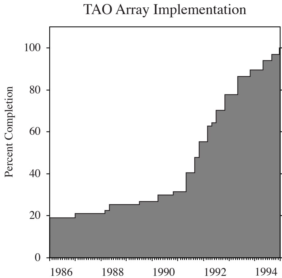
Figure 3. Rate of deployment of TOGA-TAO moorings (courtesy M. McPhaden).
