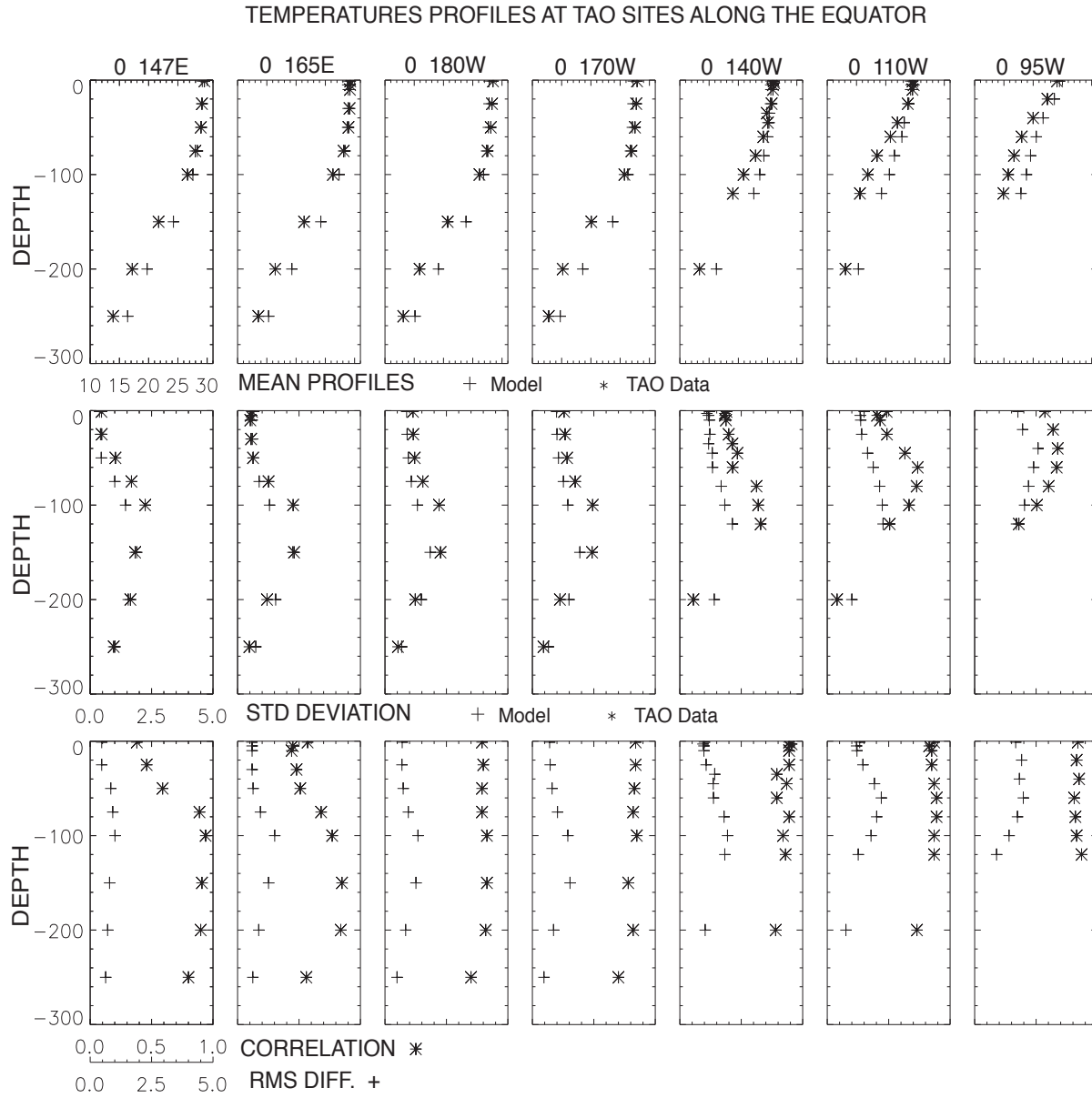
Figure 9. Comparison between model and TAO in situ temperatures along the equator at 147 E, 165 E, 180 , 170 W, 140 W, 110 W, and 95 W. The upper panel shows the mean profiles, the middle panel the standard deviation, and the lower panel the rms difference and correlation (from Vialard et al., 2001).
