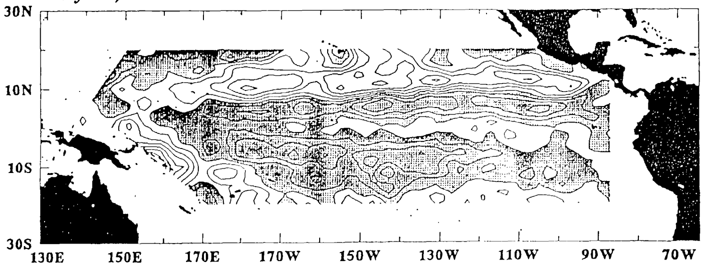
Figure 9. Sea level anomaly based on GEOSAT altimetry using the method of collinear differences. The map is constructed from approximately 2400 time series in 2 \times 1 degree (longitude x latitude) areas. Anomalies represent departures from a 1-year mean, April 1985-86. Contour interval is 4 cm, negative values shaded.
