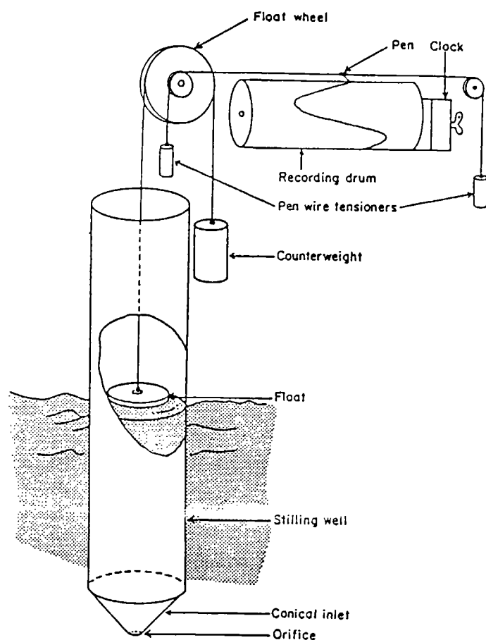
Figure 5. Basic Tide Gauge (from Manual on Sea-Level Measurement and Interpretation. 16
