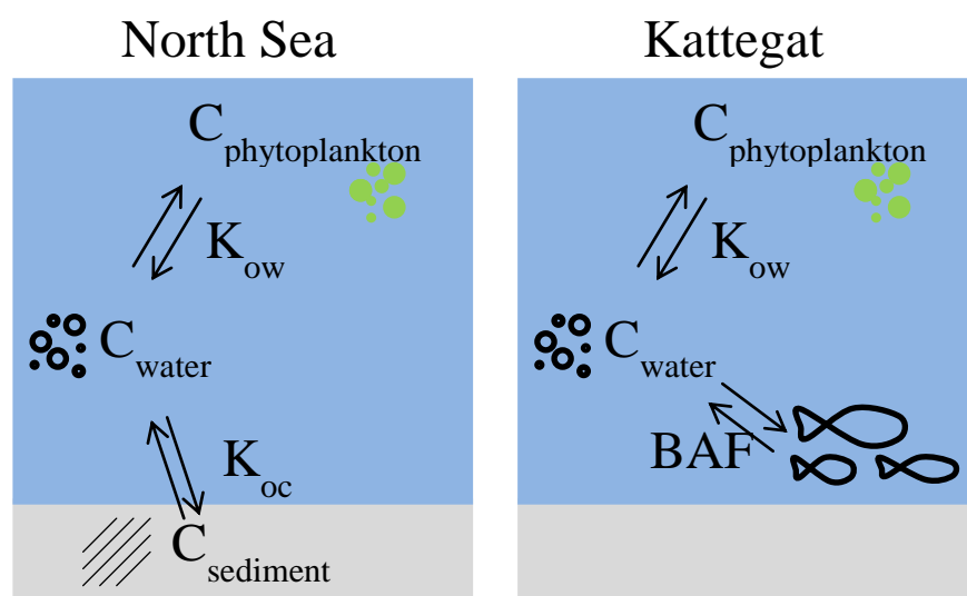
Figure D.2 Conversion between the different environmental compartments. The organic carbon – water partition coefficient ( K_{oc} ), the octanol-water partition coefficient ( K_{ow} ) and
