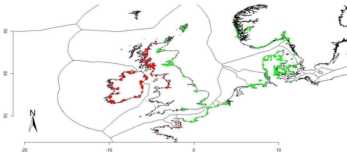
Figure B.4 Spatial distribution of the PCB mussel data in the greater North Sea (green dots) and the Celtic Sea (including west of Scotland; red dots). Information about the data selection is listed in Table B.2.
