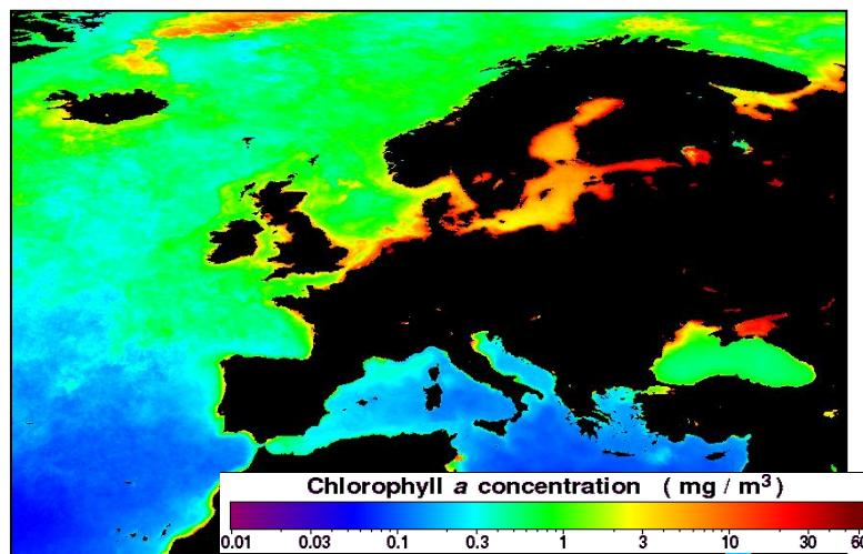
Figure 1.1 Average annual chlorophyll a concentrations in marine waters surrounding Europe in 2007. Deep blue areas have low phytoplankton productivity, orange and red areas have high productivity. Coastal environments are most productive (Redrafted from NASA-GSFC OBPG).
