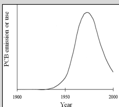
Figure 1.4 Relative emissions to the environment of polychlorinated biphenyls (PCBs) between 1900 and 2000 (Redrafted from Jones and de Voegt, 1999.)
