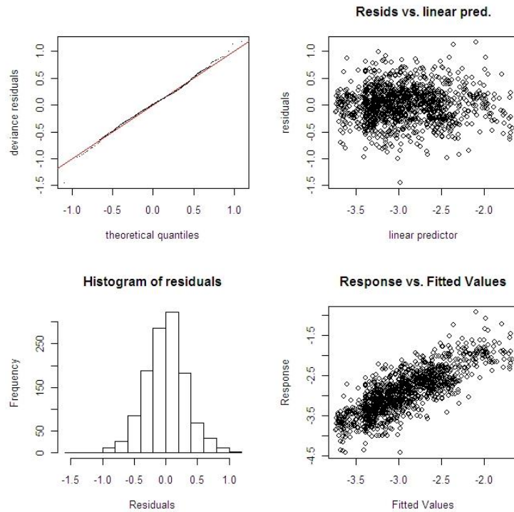
Figure A.5 Validation tools for the generalized additive mixed model that contains a smoother for time, periodicity and \log K_{oc} and two nominal variables being the sampling zone PCB cluster. The QQ plot and the histogram are used to assess normality, and the residuals versus fitted values homogeneity. The response versus fitted values should ideally show a straight line. Detection limit values are discarded in these analyses.
