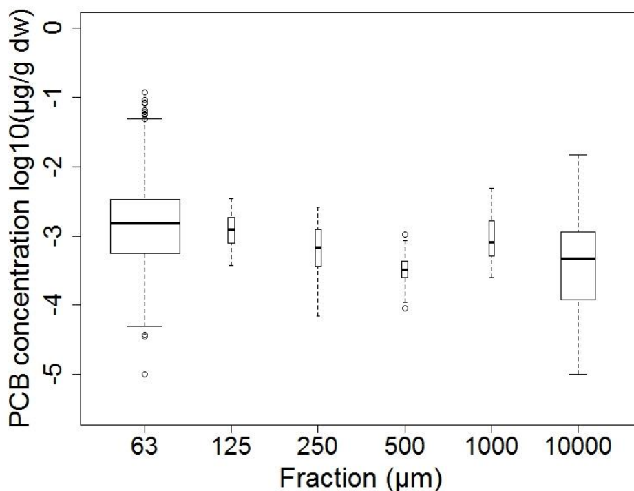
Figure A.1 Data available for each fraction (63 = fraction smaller than 63 μm; 125 = fraction smaller than 125 μm; 250 = fraction smaller than 250 μm; 500 = fraction smaller than 500 μm; 1000 = fraction smaller than 1000 μm; 10000 = fraction smaller than 10000 μm).
