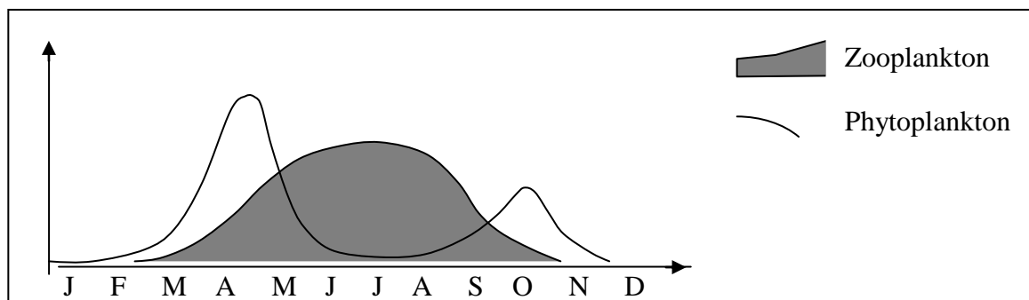
Figure 1.2 Seasonal variability of phyto- and zooplankton production in temperate marine ecosystems (Cushing, 1975).
