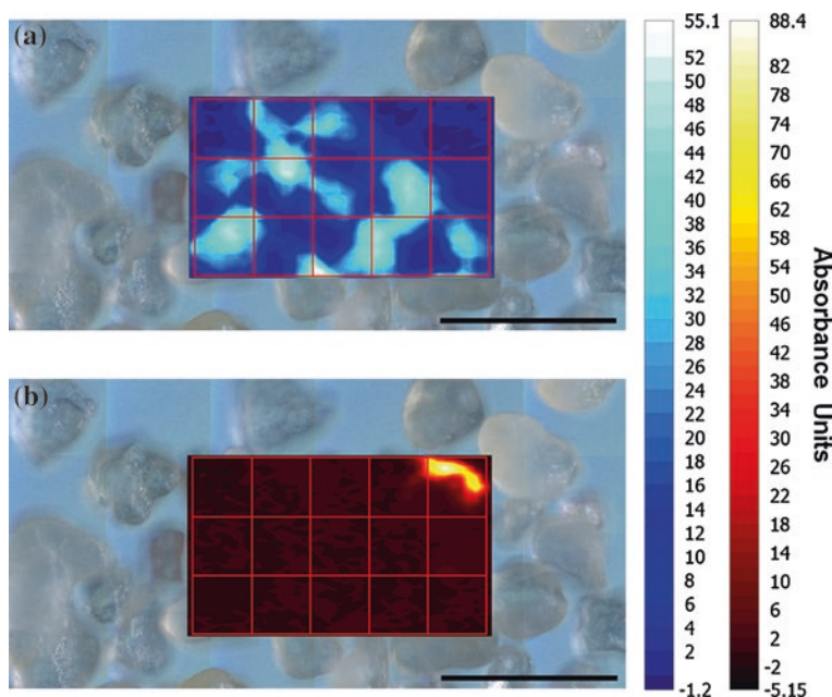
Fig. 8.7 Chemical imaging of an integration of typical spectral bands of a quartz (1931–1832 cm -1 ), b polyethylene (2981–2780 cm -1 ) in the sample Wu_Ku_Eu 4 analyzed by FPA-based micro-FTIR spectroscopy. The color scale represents the intensity of the chosen spectral bands according to peak area ( bluish color scale intensity of the peak 1,931–1,832 cm -1 ; reddish color scale intensity of the peak 2,981–2,780 cm -1 ) and clearly shows quartz particles in light blue (a) and a polyethylene particle in orange (b). Scalebars: 500 μm
