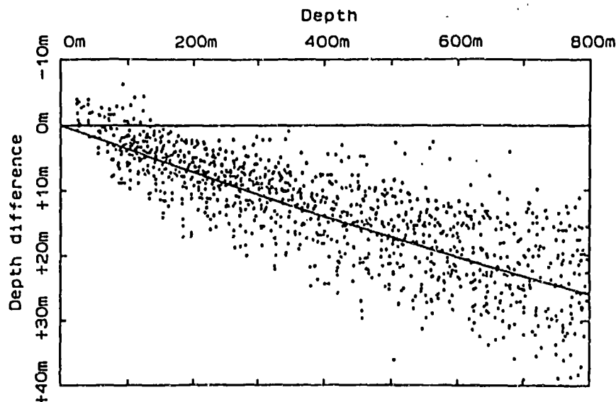
FIG. 5. Scatterplot of depth difference (ordinate) between the true depth of markers and the depth calculated from the equation provided by the XBT manufacturer, Eq. (2) (abscissa). The solid line denotes the depth difference according to the newly estimated empirical depth-time equation (3).
