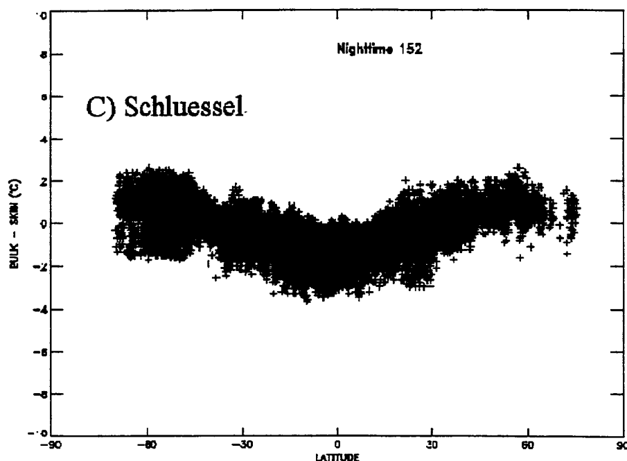
Fig. 4 Differences between the Schluessel skin SST and the SST computed by the U.S. Navoceano using buoy regressed coefficients.
