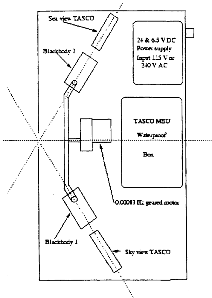
Ship of opportunity sea surface temperature radiometer C. J. Donlon March 1997
