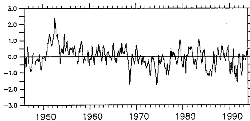
Seasonal SSTA, NW North Atlantic
