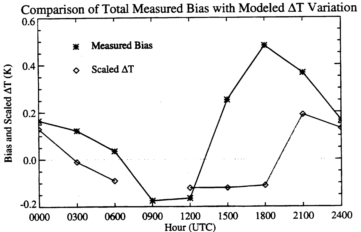
Fig. 3 Measured and simulated diurnal \bullet T variations.
