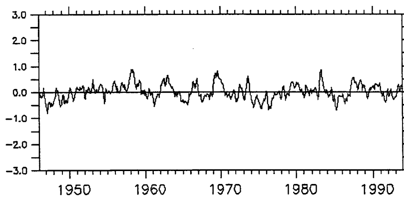
SSTA, Equatorial Atlantic
