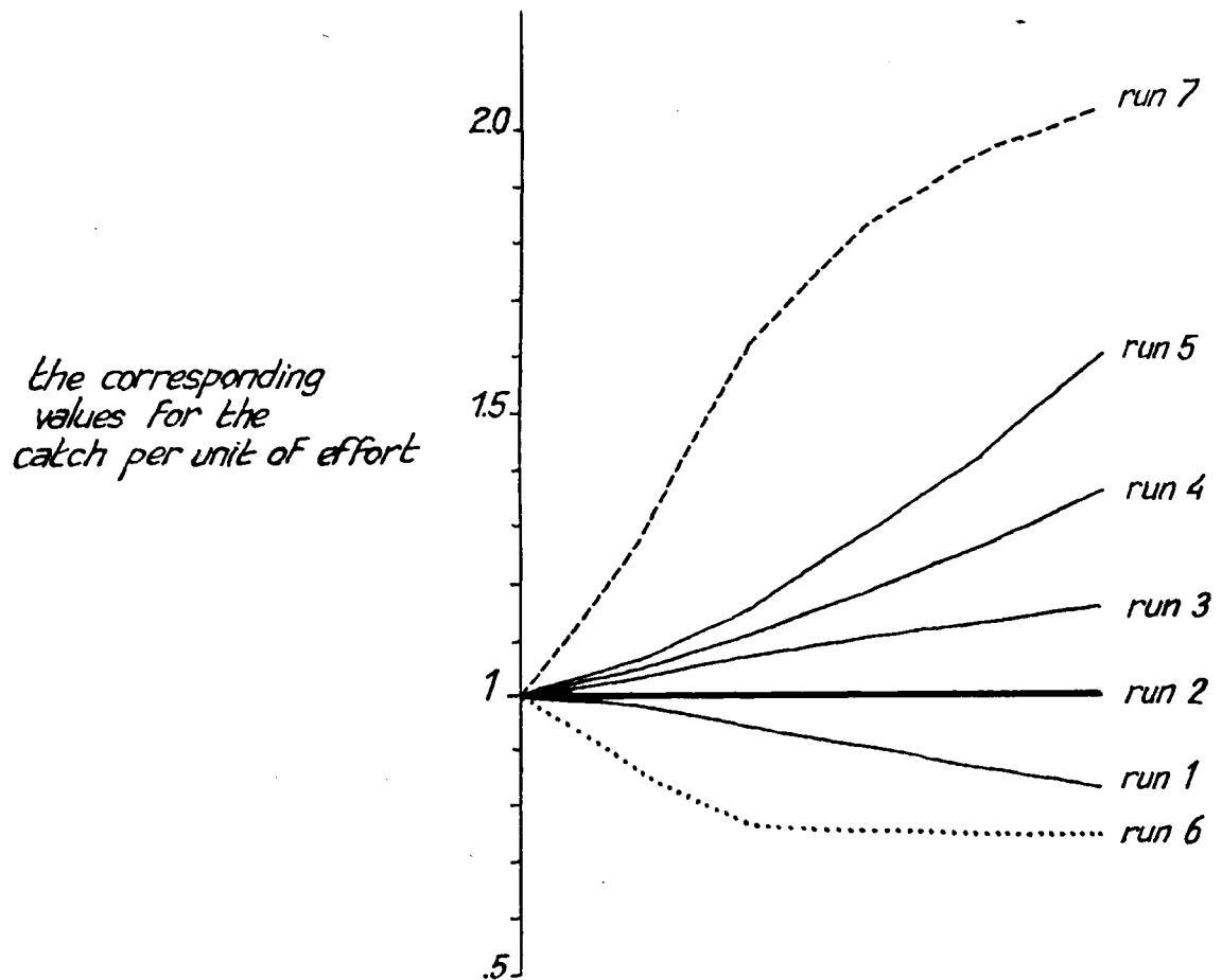
Fig. 6 North Sea Sole
