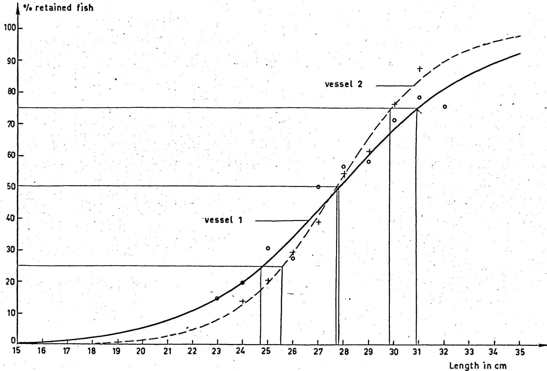
Figure 4 — Selection curves of whiting for combined hauls
