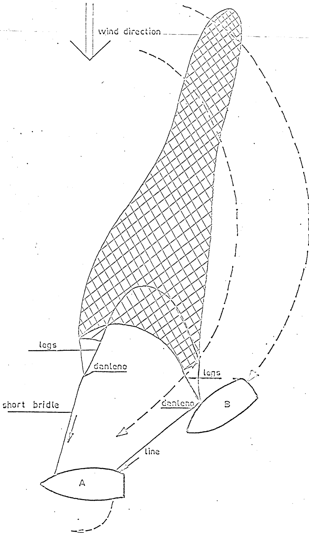
Figure 15 - Hauling: phase 4
