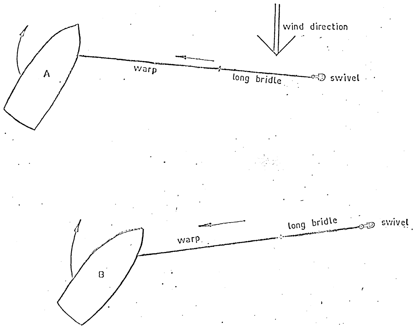
Figure 13 - Hauling: phase 2
