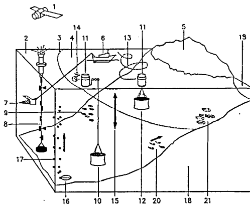
Fig. 2 : RECRUITMENT OF THE SOLE (CIRESOL, 1987)
