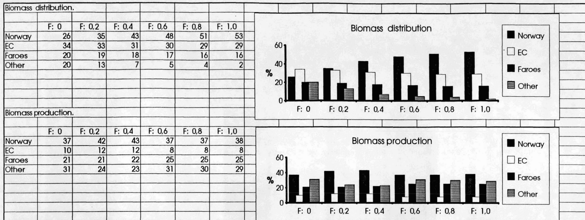
Figure 2. Biomass distribution and biomass production indices of blue whiting by economic zones as a function of the fishing mortality F . For further explanation, see text.
