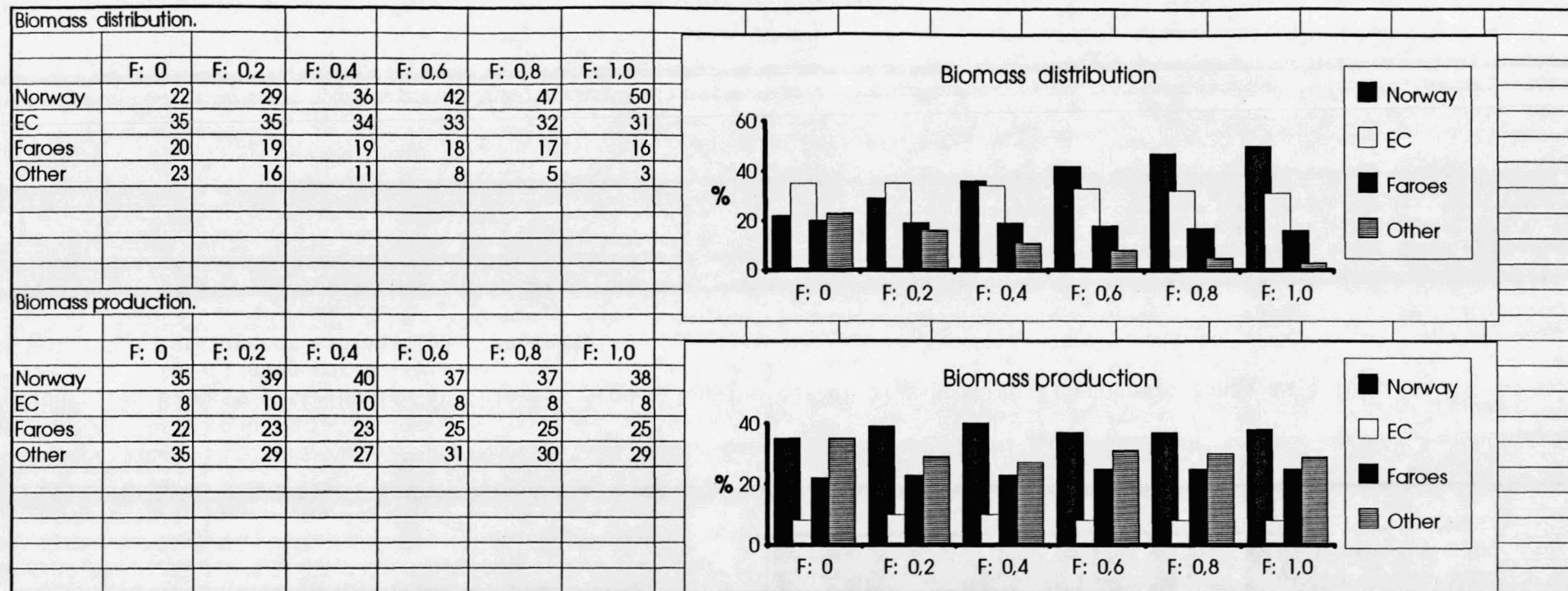
Figure 3. Biomass distribution and biomass production indices of blue whiting by economic zones as a function of the fishing mortality F . The K -factor (Tables 1 and 2) for ages 3+ = 2. For further explanation, see text.
