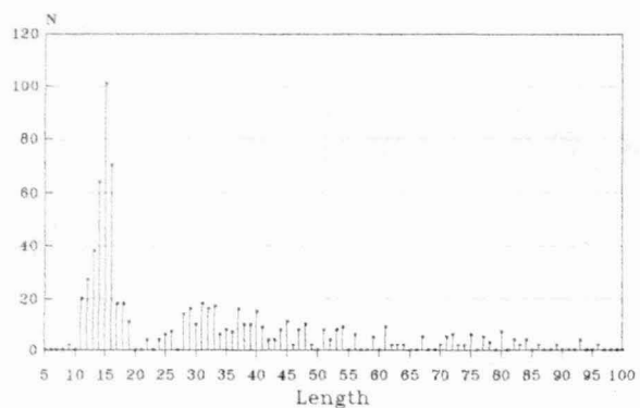
Fig. 6 Length distributions of white monk fish.
