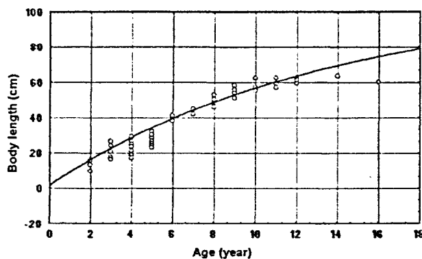
Figure 4: Von Bertalanffy growth curve for females.
