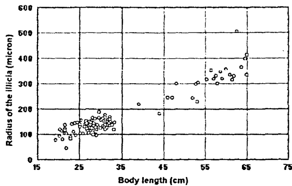
Figure 2: Relation between the body length (C) and the radius of the Illicium (I) for females.
