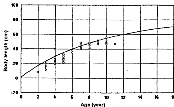
Figure 5: Von Bertalanffy growth curve for males.
