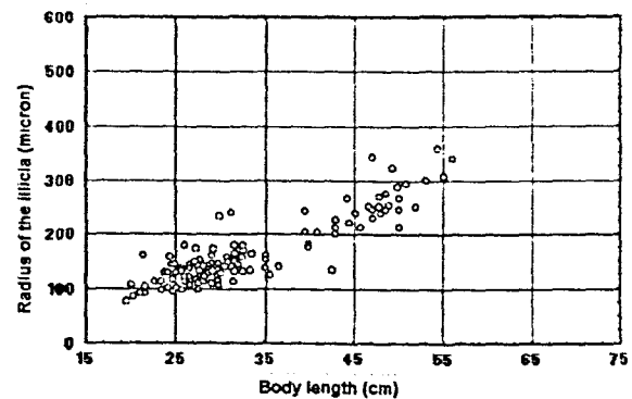
Figure 3: Relation between the body length (C) and the radius of the Illicium (I) for males.
