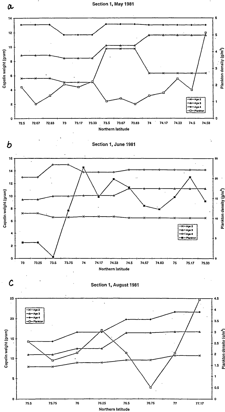
Figure 3. Plots of plankton biomass and individual mean weight by age group of capelin along section I 1981. a) May, b) June, c) August.
