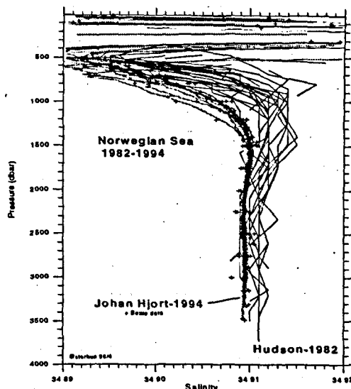
Figure 3. Salinity profiles along the CCS Hudson 1982 and R/V Johan Hjort 1994 sections in the Norwegian Basin.
