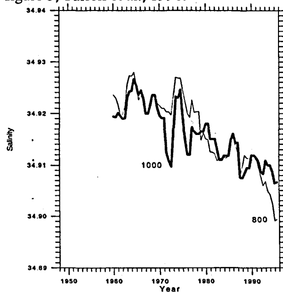
Figure 5. Time series of the salinity at 800 and 1000 m depth in the Faroe-Shetland Channel.
