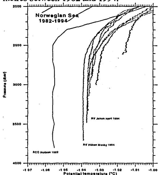
Fig. 2. Temperature profiles from 1982 and 1994 of the adiabatic deep water in the central part of the Norwegian Basin.
