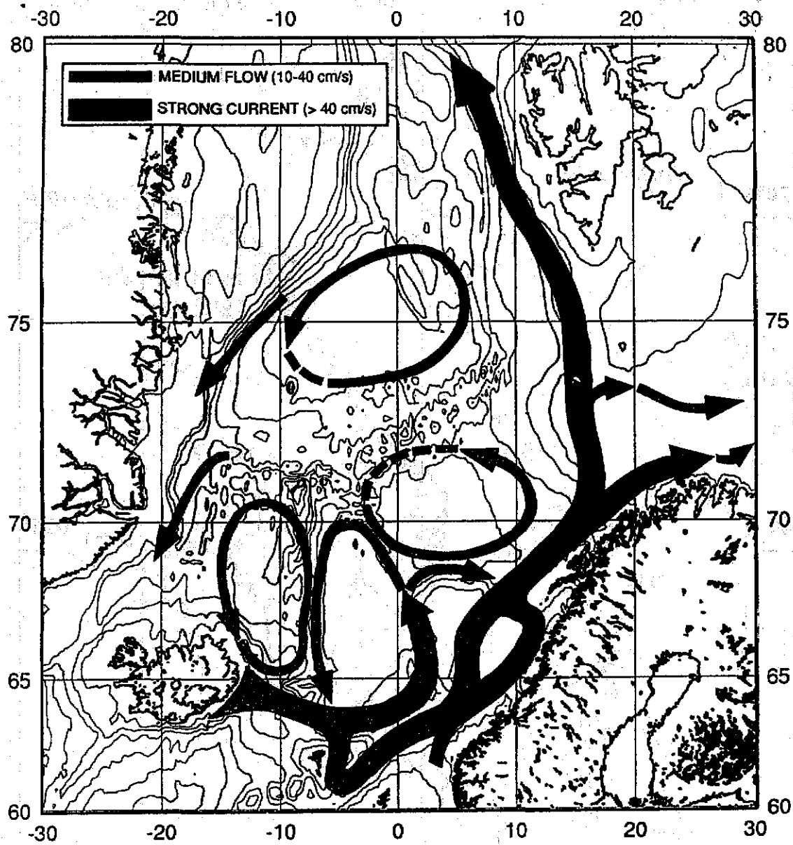
Fig.18. Schematic of surface circulation in the Norwegian Sea derived from Lagrangian drifter data. The East Greenland Current is not depicted due to ice coverage. From Poulain et al. 1996.
