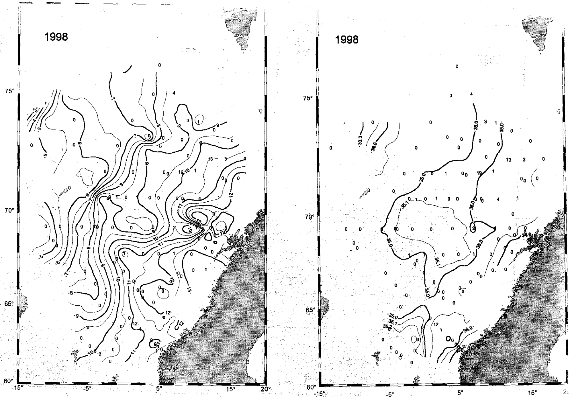
Fig. 7. Trawl stations in 1998 without (0) and with nr of smolts (1,2, etc) in relation to temperature (left panel) and salinity (right panel) isotherms at 5 m depth in the Norwegian Sea in July - 3 d week of August.
