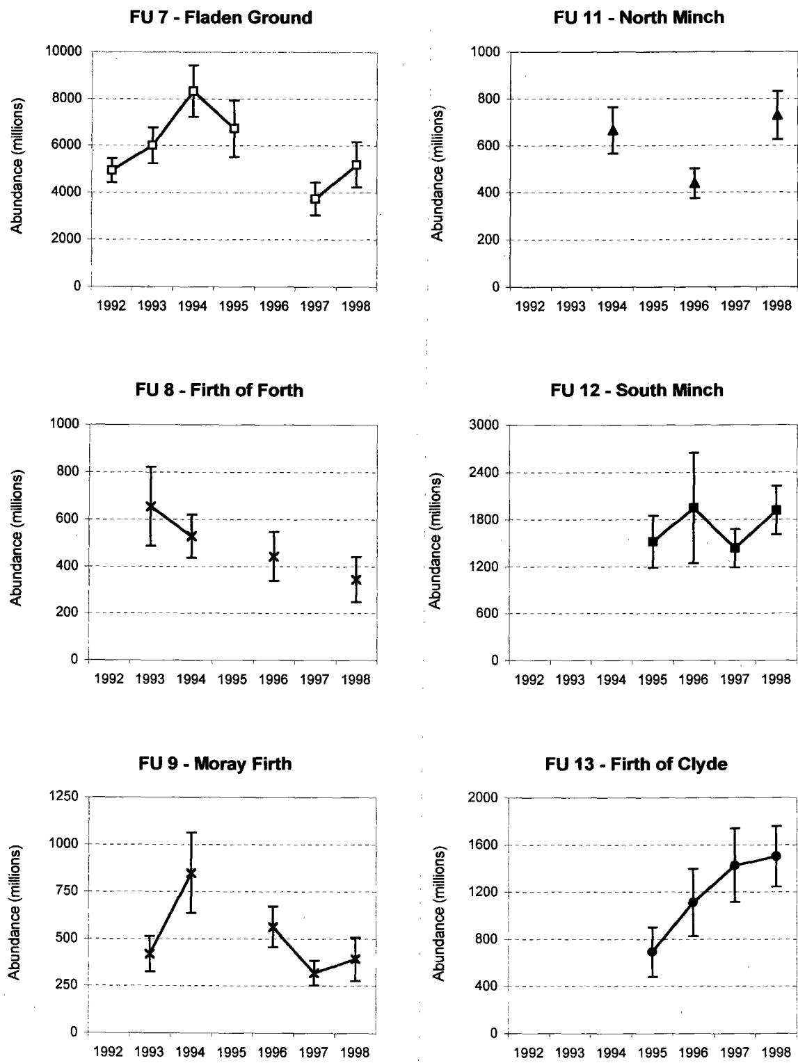
Figure 7.2. - Trends in abundance (in millions) of Nephrops in various Scottish stocks, estimated from underwater TV surveys, 1992-98. Vertical bars indicate 95 % confidence intervals.
