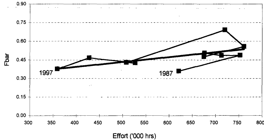
Figure 5.16.10. - Bay of Biscay (FUs 23-24): Effort and Fbar, and relationship between them, for males and females.
