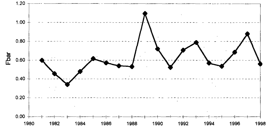
Fbar 3-8 - XSA estimates
