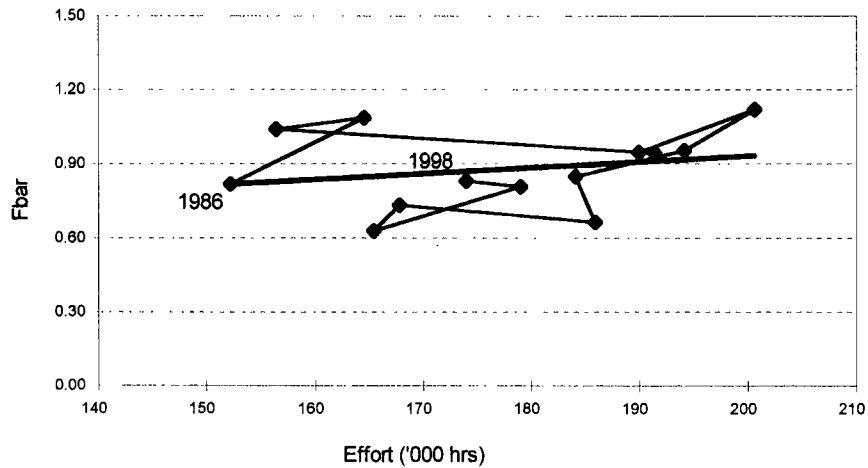
Figure 5.12.13. - Irish Sea West (FU 15): Effort and Fbar, and relationship between them, for males and females.
