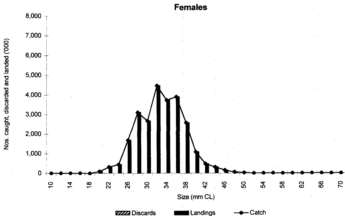
Figure 9.10. - Porcupine Bank (FU 16): Length frequency distributions (in '000) of Nephrops caught, discarded and landed. Males and females shown separately.
