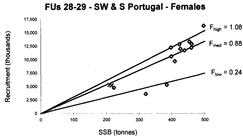
Figure 8.3. (f) - Stock-recruitment plots and associated BRPs. Lines represent ratios of recruitment to SSB corresponding to the BRP estimates. SSB and recruitment estimates for the last two years (marked as x) were excluded from estimation of BRPs.
