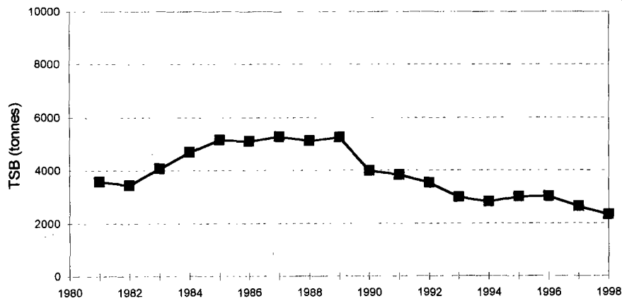
TSB - XSA estimates
