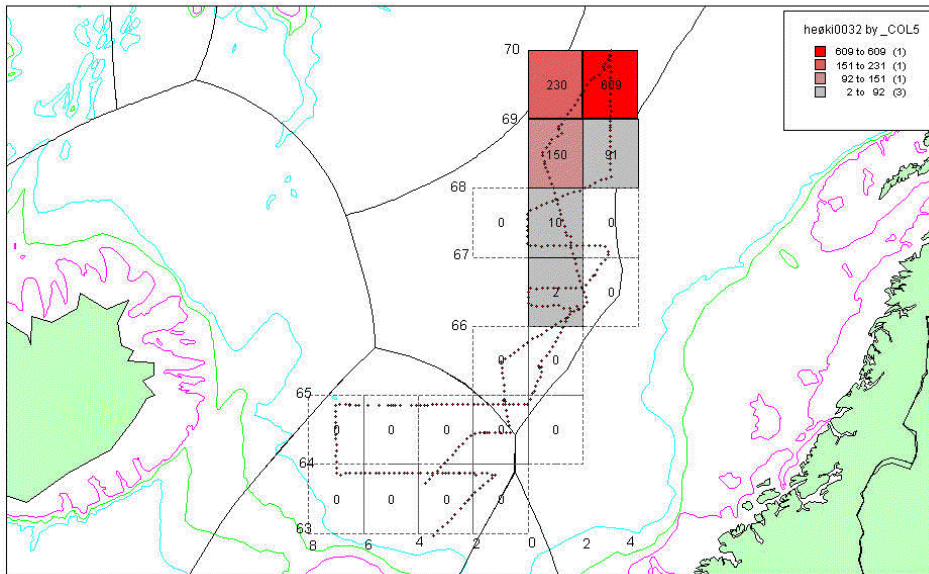
0032: Mean S_A -values in statistical squares (Herring)
