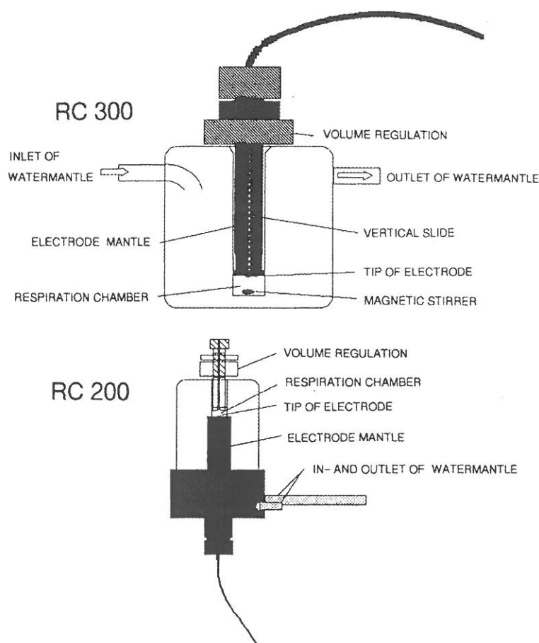
Figure 1. The RC 300 and RC 200 respiration vials. The drawings are not to relative size. Both respiration chambers have a diameter of 1.5 cm; diameter x height of the vials is 5 cm x 5.6 cm and 3,7 cm x 7,7 cm for the RC 300 and RC 200, respectively.
