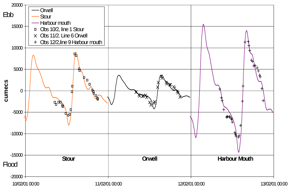
Figure 6.3 Calibration of 2D model (source: HR Wallingford)
