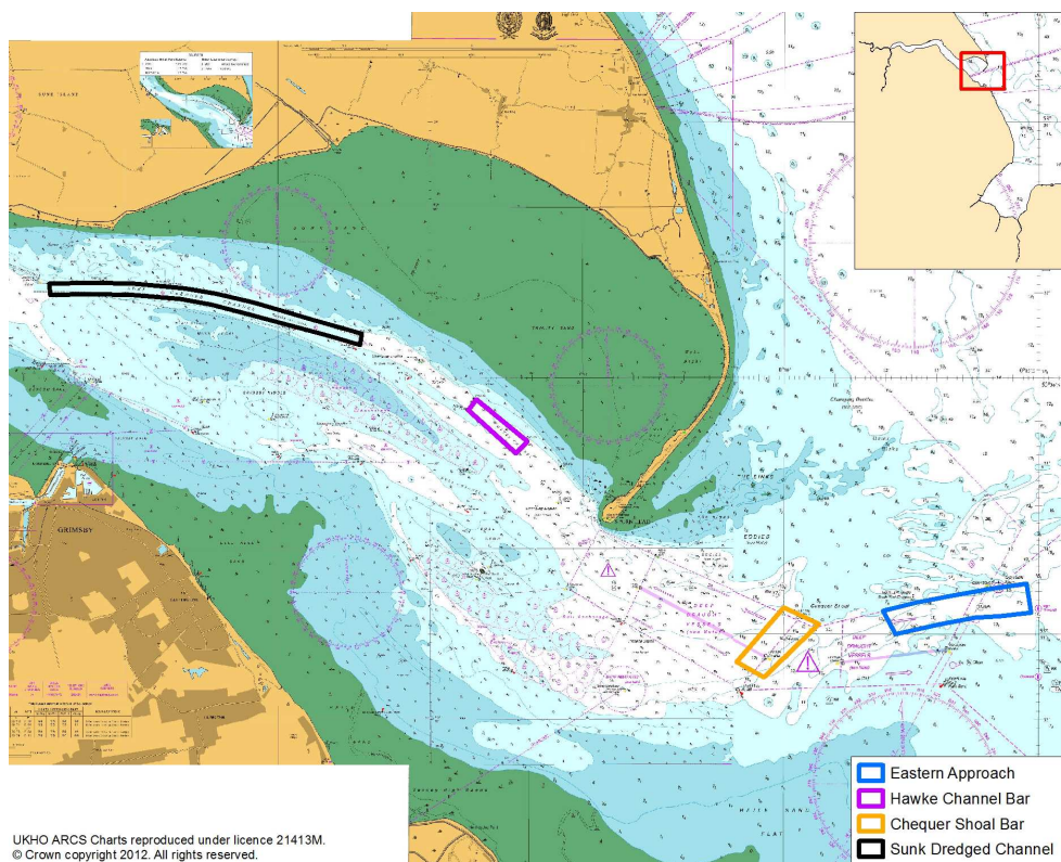
Figure 4.1 Proposed dredging locations for the Immingham Oil Terminal Approach Channel Deepening project (source: ABPmer, 2009)
