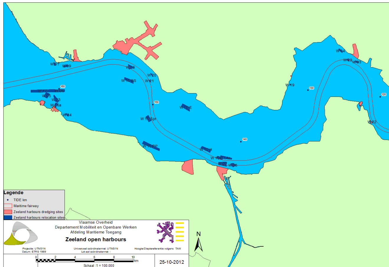
Map 5 Dredging and relocation sites for the Zeeland open harbours
