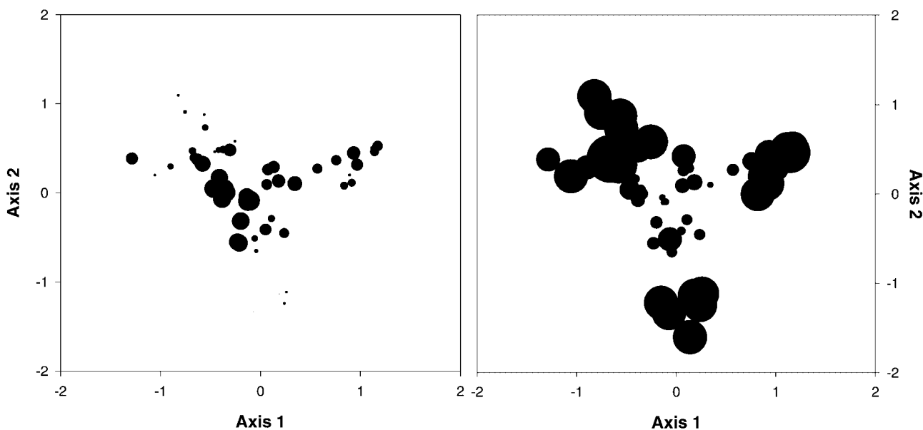
Fig. 5. – Superpositioning of the abundance (left) and sex-ratio proportion males:females (right) on the MDS-plot (fig. 3).
