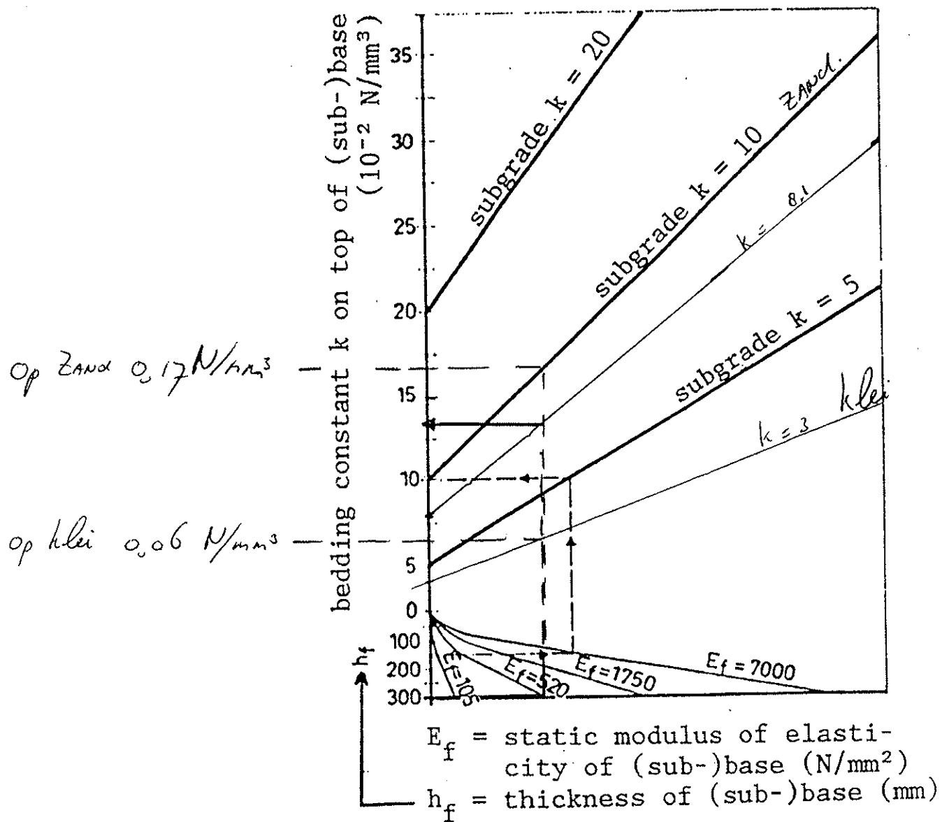
Figure 4. Nomograph for the determination of the k -value of (sub-)base layer (1).
