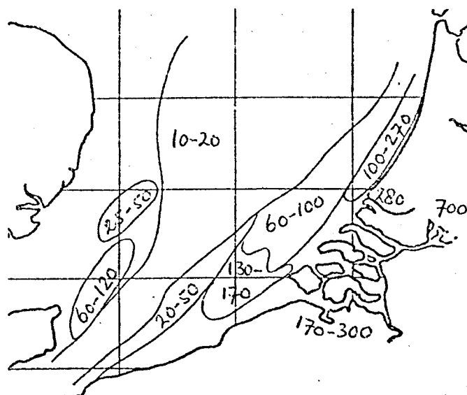
Fig.4d. Particulate leacheable iron in µg per liter.
