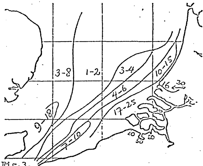
Fig.3. Weight of suspended matter obtained after filtration through 0.45 \mu m pore size Millipore filters, in mg per liter.
