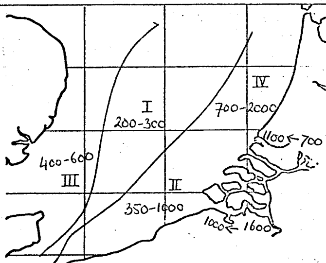
Fig.5. Different regions with different characteristic particulate leacheable manganese concentrations in µg Mn per g.
