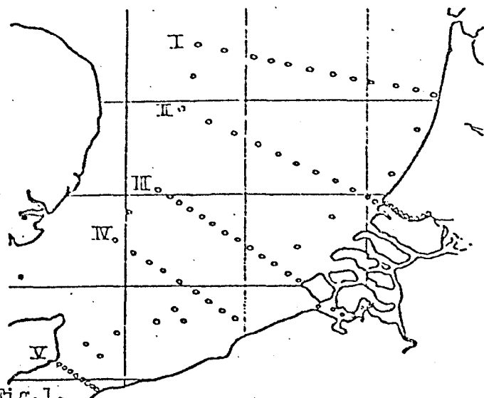
Fig.1. Net of sampling stations. Series I: off Ymuiden; II: off the river Rhine; III: off the river Scheldt; IV: off Ostend; V: Straits of Dover.
