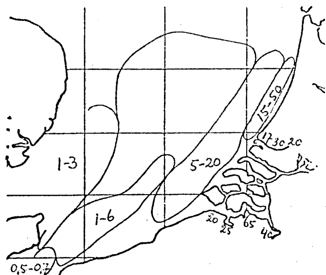
Fig.4c. Particulate leacheable manganese in µg per liter.
