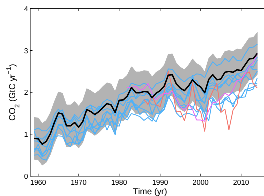
Figure 7. Comparison of the anthropogenic atmosphere–ocean CO 2 flux shows the budget values of S_{OCEAN} (black), individual ocean models before normalisation (blue), and the two ocean-data-based products (Rödenbeck et al., 2014, in salmon and Landschützer et al., 2015, in purple; see Table 6). Both data-based products were adjusted for the pre-industrial ocean source of CO 2 from river input to the ocean, which is not present in the models, by adding a sink of 0.45 GtC yr -1 (Jacobson et al., 2007) so as to make them comparable to S_{OCEAN} . This adjustment does not take into account the anthropogenic contribution to river fluxes (see Sect. 2.7.2).
