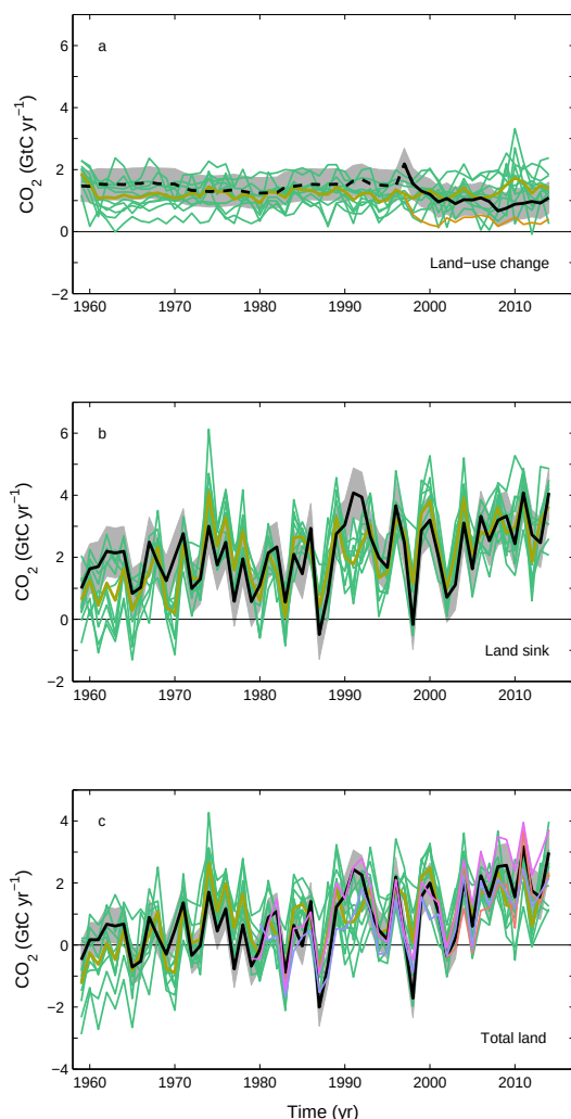
Figure 6. (a) Comparison of the atmosphere–land CO 2 flux showing budget values of E_{LUC} (black). CO 2 emissions from land-use change showing individual DGVM results (green) and the multi-model mean (olive), as well as fire-based results (orange); land-use-change data prior to 1997 (dashed black) highlight the start of satellite data from that year. (b) Land CO 2 sink ( S_{LAND} ; black) showing individual DGVM results (green) and multi-model mean (olive). (c) Total land CO 2 fluxes (b–a) from DGVM results (green) and the multi-model mean (olive); atmospheric inversions of Chevallier et al. (2005; MACC, v14.2) (purple), Rödenbeck et al. (2003; Jena CarboScope, s81_v3.7) (violet), and Peters et al. (2010; Carbon Tracker, vCTE2015) (salmon) (see Table 6); and the carbon balance from Eq. (1) (black). In (c) the inversions were adjusted for the pre-industrial land sink of CO 2 from river input, by adding a sink of 0.45 GtC yr -1 (Jacobson et al., 2007). This adjustment does not take into account the anthropogenic contribution to river fluxes (see Sect. 2.7.2).
