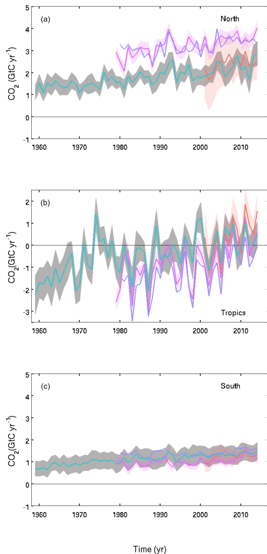
Figure 8. Atmosphere-to-surface \text{CO}_2 flux ( S_{\text{OCEAN}} + S_{\text{LAND}} - E_{\text{LUC}} ) by latitude bands for the (a) north (north of 30^\circ\text{N} ), (b) tropics ( 30^\circ\text{S} – 30^\circ\text{N} ), and (c) south (south of 30^\circ\text{S} ). Estimates from the combination of the multi-model means for the land and oceans are shown (turquoise) with \pm 1\sigma of the model ensemble (in grey). Results from the three atmospheric inversions are shown in purple (Chevallier et al., 2005; MACC, v14.2), violet (Rödenbeck et al., 2003; Jena CarboScope, s81_v3.7), and salmon (Peters et al., 2010; Carbon Tracker, vCTE2015); see Table 6.
