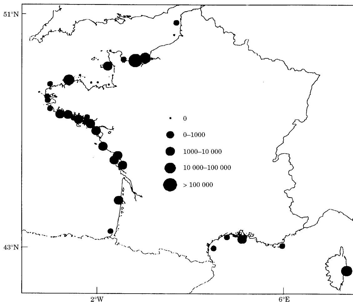
Figure 7. Map showing maximum cell counts for Dinophysis sp. (in classes) per site for 1995.
