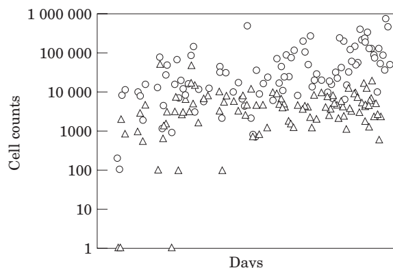
Figure 2. Time-series data of cell counts for two groups of species at a single station as an example of maintaining precision in space and time while aggregating data over species. Coastal species (○); benthic species (△).
