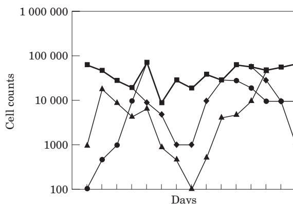
Figure 4. As Fig. 3, but highlighting the maximum cell counts observed at the site on each date as an example of maintaining precision in time while aggregating over space and species. Station 1 (—●—); station 2 (—◆—); station 3 (—▲—); maximum (—■—).
