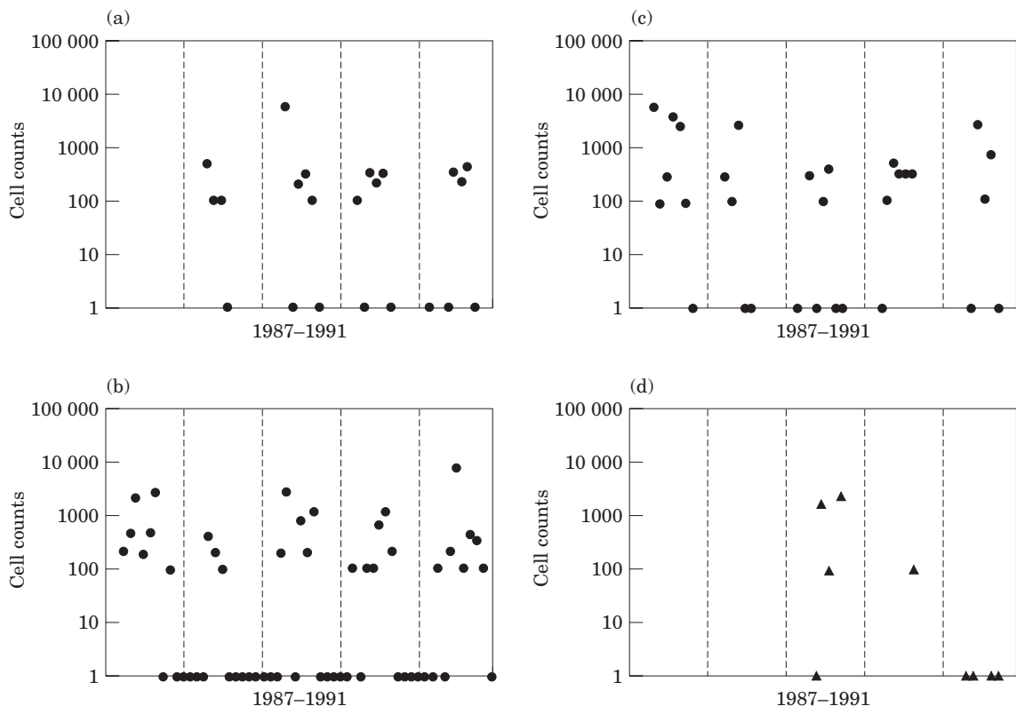
Figure 6. Maximum cell counts for two toxic phytoplankton species by subsite and month over 5 years as an example of aggregating over time and space while maintaining genus or species information. (a) Dinophysis sp.—sub-site 1; (b) Dinophysis sp.—sub-site 2; (c) Dinophysis sp.—sub-site 3; (d) Alexandrium minutum —sub-site 2.
