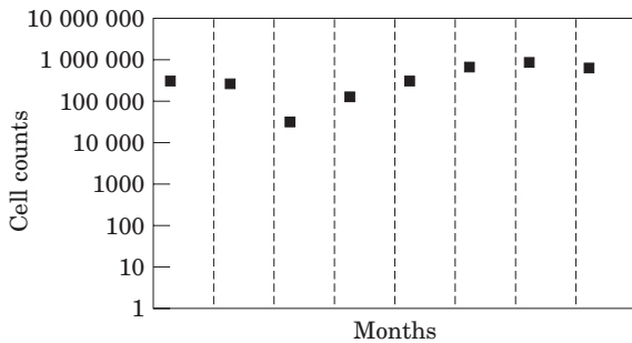
Figure 5. Maximum cell counts for one group of species observed at a particular site within a particular month as an example of aggregating in three dimensions.
