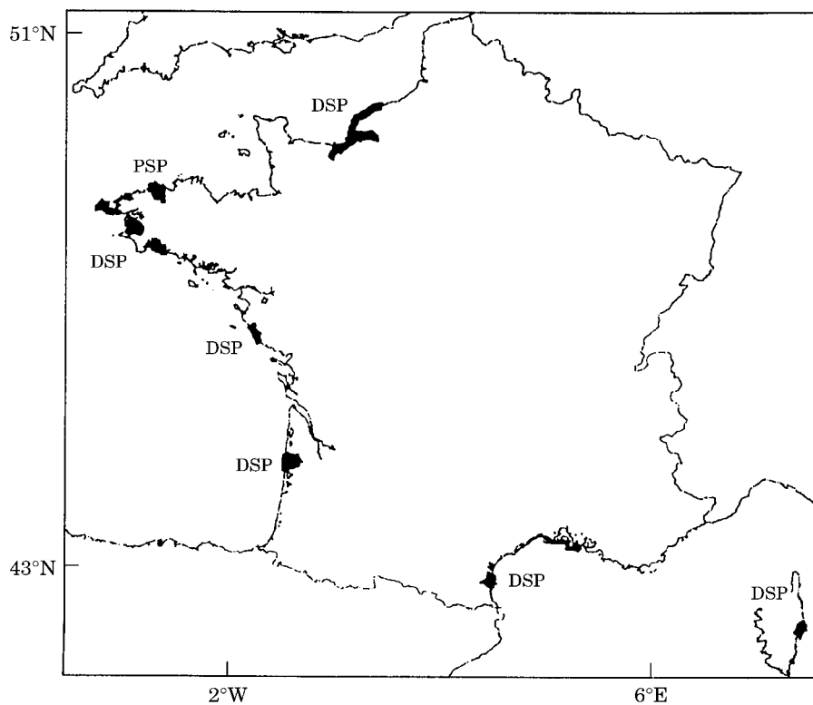
Figure 9. Areas temporarily closed to shellfish fisheries because of the presence of DSP or PSP toxins in 1995.
