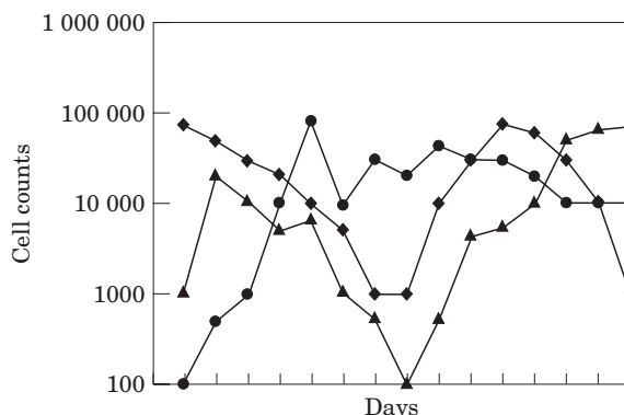
Figure 3. Time-series data of cell counts for one group of species at three stations belonging to one site as an example of maintaining precision in space and time while aggregating data over species. Station 1 (—●—); station 2 (—◆—); station 3 (—▲—).
