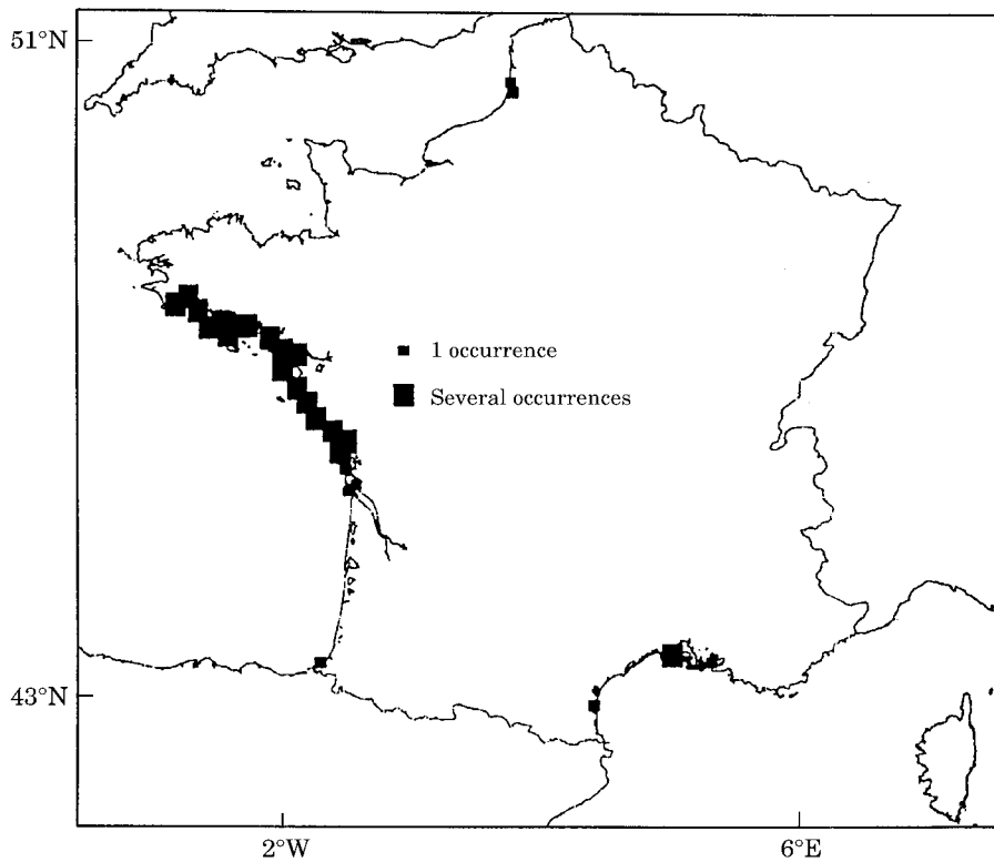
Figure 8. Frequency of occurrence of Noctiluca scintillans blooms per site for 1984–1992.
