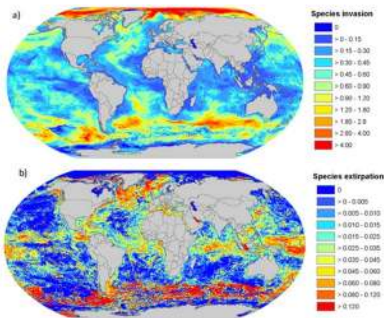
Figure 4. Projected intensity of species invasion (a) and local extinction (b) by 2050 relative to 2000 (10-year average) under the SRES A1B scenario. (Redrawn from Cheung et al. , 2009).
