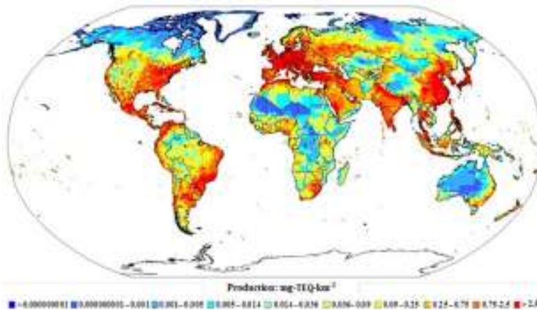
Figure 3. Global production of dioxin as toxic equivalents of 2,3,7,8-tetrachlorodibenzo- p -dioxin spatialized over the earth's surface with emissions based on an environmental Kuznets curve.
