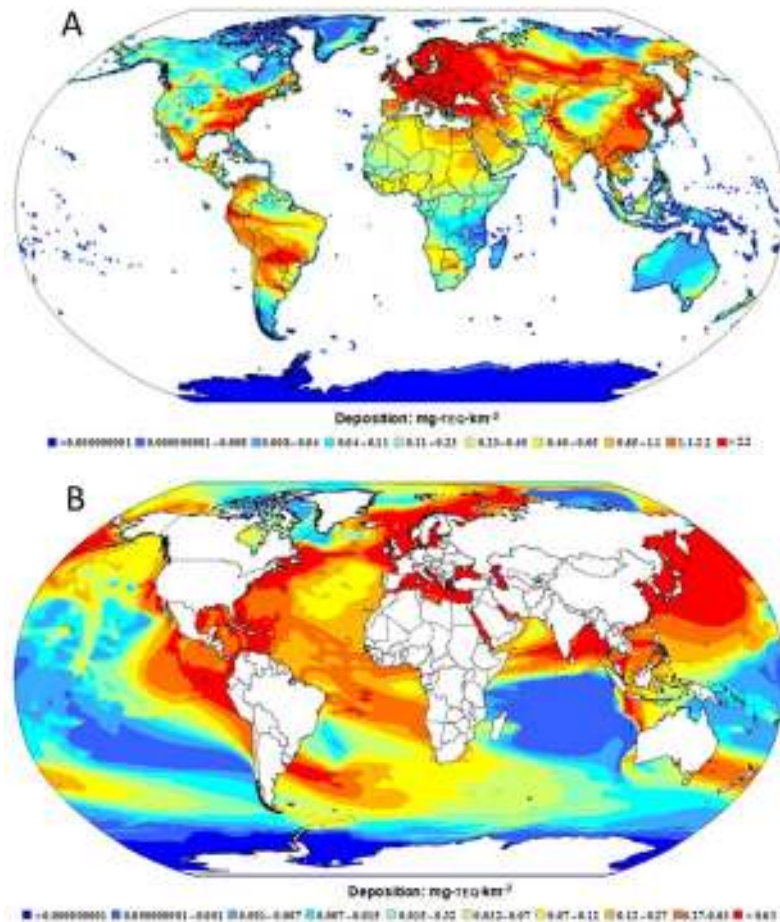
Figure 4. Deposits of dioxin presented as toxic equivalents of 2,3,7,8-tetrachlorodibenzo- p -dioxin after simulating one year of transport processes of global atmospheric emissions, to A) land; and B) oceans.
