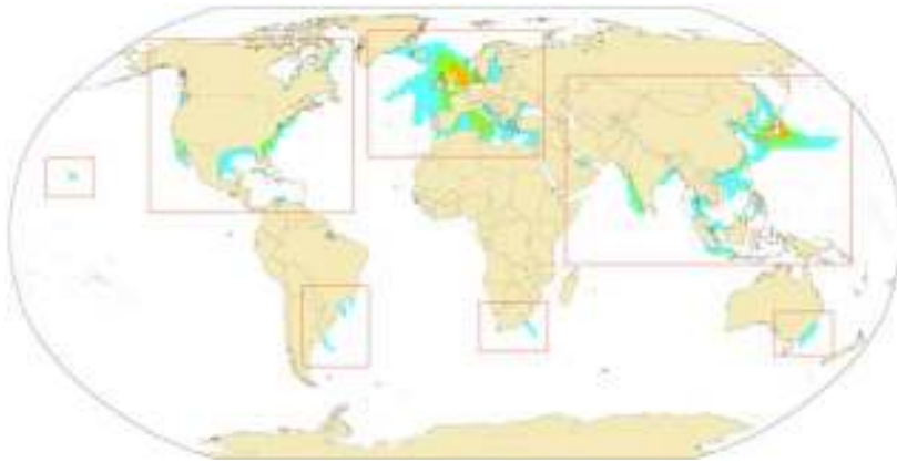
Figure 1. Predicted relative dioxin concentration in small pelagic fishes. Scale is from white to light blue to green, yellow and orange (adapted from Figure 9 in Christensen and Booth, 2006). Note high concentrations in the waters around Asia, Europe and North America, versus lower concentrations in South America, Africa and Australia.
