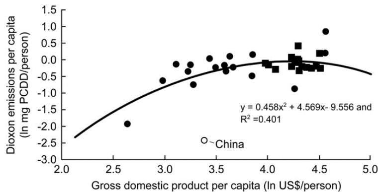
Figure 2. Environmental Kuznets curve used to estimate countries' per capita dioxin emissions. Original data used in Baker and Hites (2000) are shown in square symbols (■), new data are shown in circles (●) with China (○) omitted from analysis.
