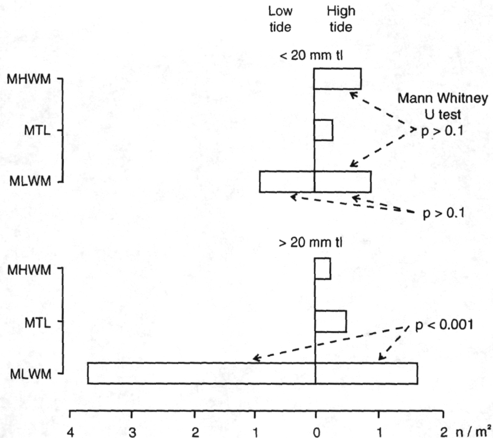
Fig. 4: Densities of Crangon crangon taken in beam trawls at MLWM at low tide and at MLWM, MTL and MHWM at high tide. Mean values are shown separately for small (< 20 mm t.l.) and large (> 20 mm t.l.) specimens in 20 samples at each tidal level over a 10 month sampling period (Original).
