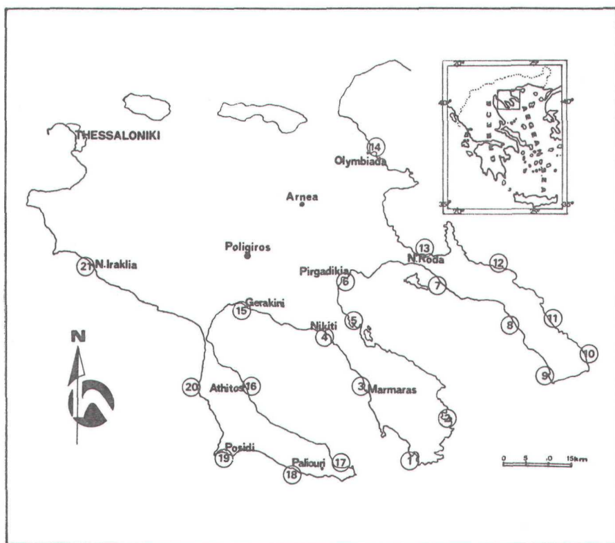
FIG. 1 Map of Chalkidiki Peninsula, indicating the sampling stations.
