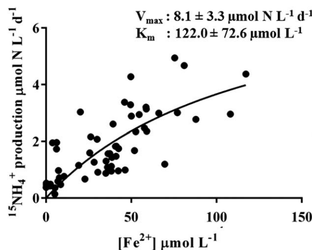
Fig. 7. Michaelis-Menten kinetics of DNRA rate (as ^{15}\text{NH}_4^+ production) against the initial \text{Fe}^{2+} concentration in all slurry experiments (excluding those with acetate addition) \pm SD.
