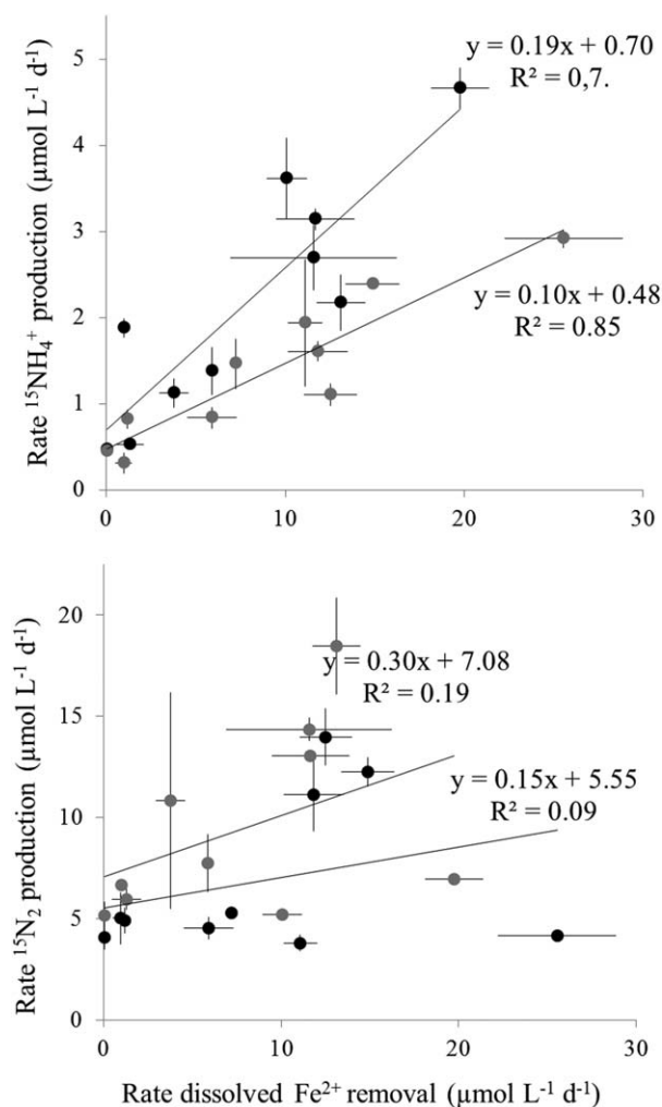
Fig. 6. Correlation between average rates of \text{Fe}^{2+} removal and ^{15}\text{NH}_4^+ production (top panel) and ^{15}\text{N}_2 production (bottom panel) in slurry incubations with ^{15}\text{N} -nitrate (black dots) and ^{15}\text{N} -nitrite additions (grey dots) from all sites investigated. No rates are included from experiments with ^{15}\text{N} -nitrate and acetate addition.
