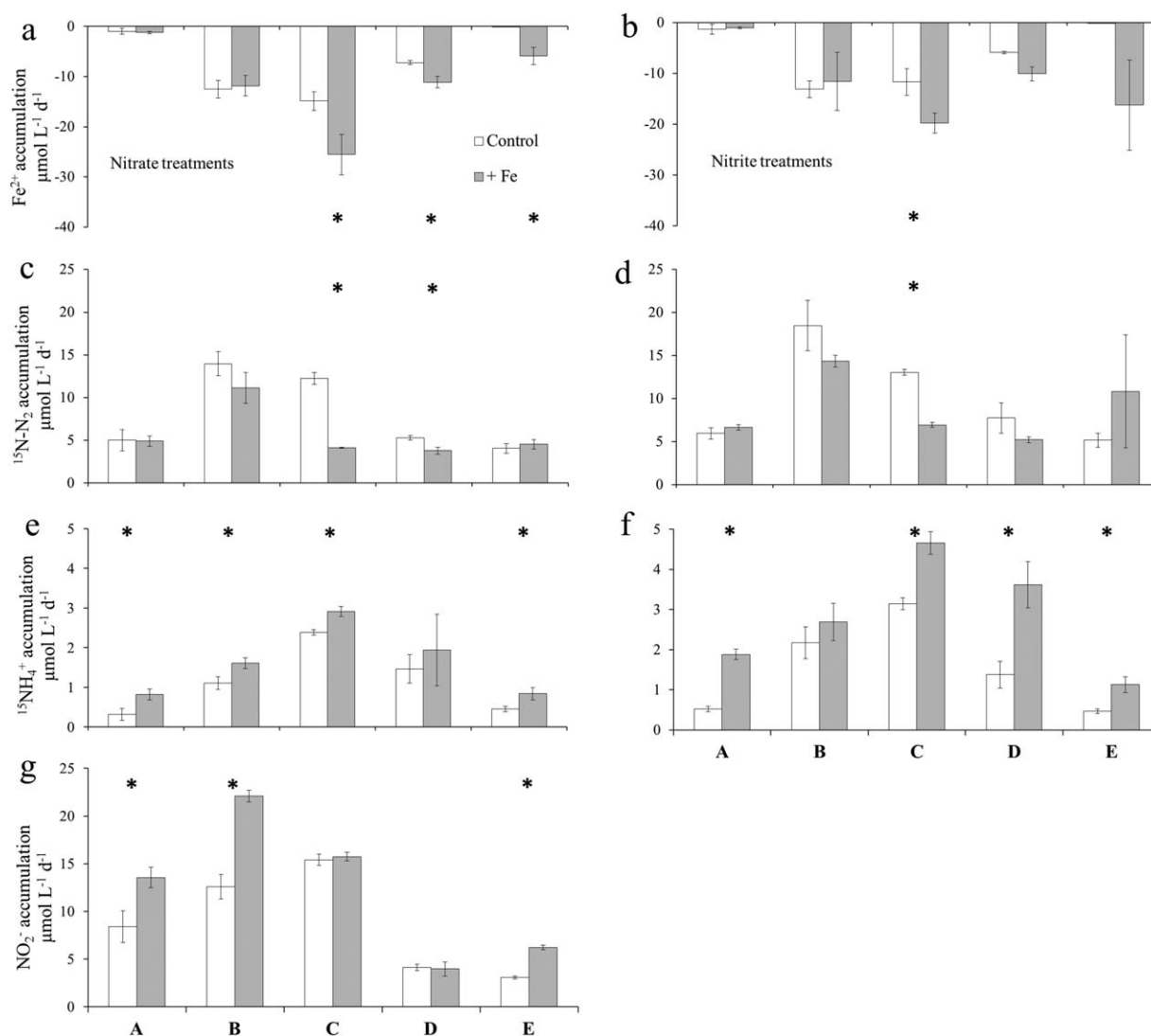
Fig. 4. Average rates of \text{Fe}^{2+} consumption (a, b) and ^{15}\text{N-N}_2 (c, d), ^{15}\text{NH}_4^+ (e, f) production and \text{NO}_2^- accumulation (g) rates from dilute slurry experiments ( \mu\text{mol N} or \text{Fe}^{2+} \text{ L slurry}^{-1} \text{ d}^{-1} ). Asterisks (*) above bars show significant ( p > 0.05 , t -test) differences between control and iron-amended slurries. Bars show SD ( n = 3 ).
