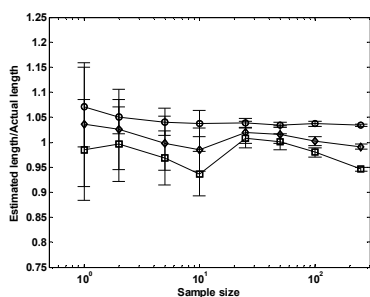
Figure 2. Ratio of measured length to actual length for three estimators as a function of sample size. \diamond – equation (4); \circ – equation (7); \square – equation (8).
