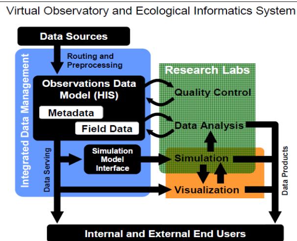
Figure 1. High level architectural view of VOEIS
