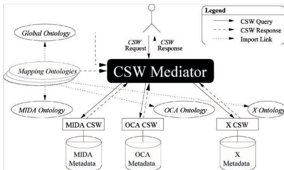
Figure 5: Ontology-based CSW mediation architecture.
