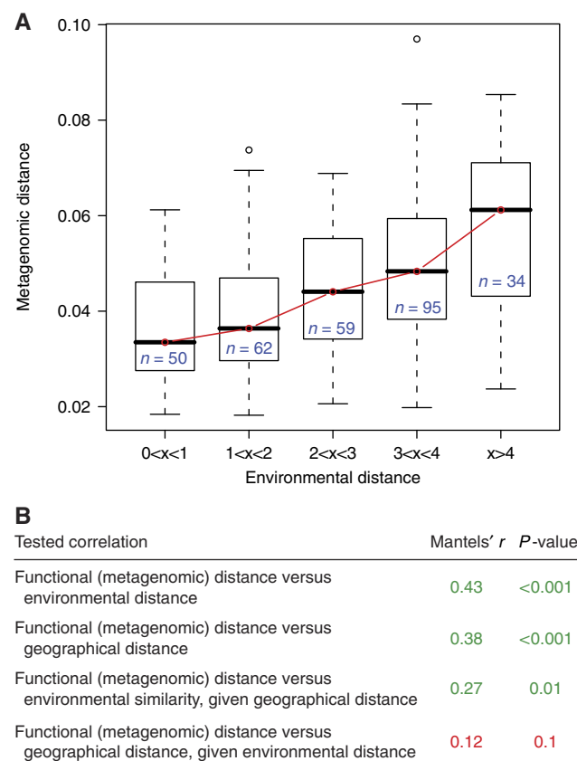
Figure 2 The role of environment in the biogeography of functional traits. (A) Coupling of metagenomic distance between samples (measured using KEGG metabolic pathway composition; see Materials and methods) with difference in climatological conditions, identifying climate as a primary determinant of function dispersion. (B) (Partial) Mantel tests (see Materials and methods) showing that this increase is not due to indirect effects, such as the similarity in environmental conditions between geographically close samples.
