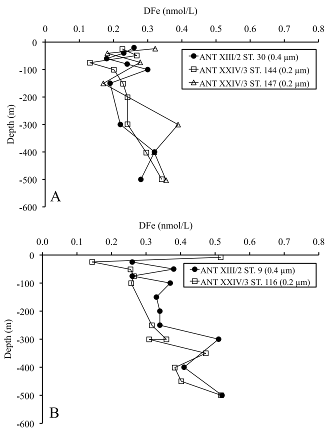
Figure 2. Compatibility of DFe-0.4 \mu\text{m} and DFe-0.2 \mu\text{m} data. (a) Vertical profiles of DFe-0.4 \mu\text{m} at ANT XIII/2 station 30 ( 63^{\circ}40'S , 0^{\circ}00'E ) (this study) and DFe-0.2 \mu\text{m} at ANT XXIV/3 stations 144 ( 63^{\circ}00'S , 0^{\circ}00'E ) and 147 ( 63^{\circ}58'S , 0^{\circ}00'E ) [Klunder et al. , 2011]. (B) Vertical profiles of DFe-0.4 \mu\text{m} at ANT XIII/2 station 9 ( 54^{\circ}00'S , 0^{\circ}00'E ) (this study) and DFe-0.2 \mu\text{m} ANT XXIV/3 station 116 ( 54^{\circ}00'S , 0^{\circ}00'E ) [Klunder et al. , 2011].
