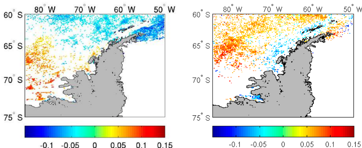
Figure 3.17.13 Trends in phytoplankton abundance (left, Chl a g\ m^{-2} ) and cell size (right, % cells greater than 20 \mu m ) in the West Antarctic Peninsula region, 1997 - 2012. Pixels indicate trends significant at p < 0.00X . Data derived from the MODIS-X ocean colour sensor. by Maria Kavanaugh, (WHOI)
