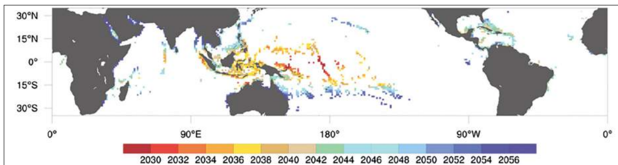
Figure 3.8.7 Global projections of the year annual severe bleaching conditions start for all reef locations under Representative Concentration Pathway (RCP) 8.5. After van Hooidonk et al. (2014).
