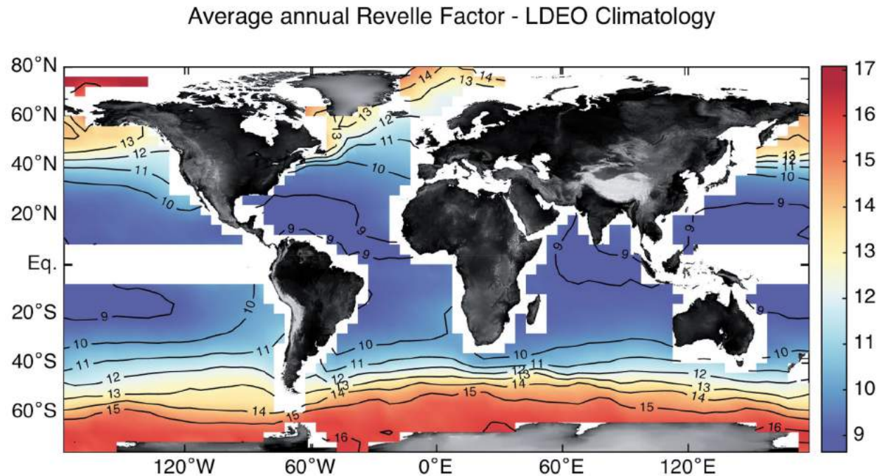
Figure 4.2.6 Annual average of Revelle Factor – this describes the capacity of the surface ocean to absorb additional carbon dioxide from the atmosphere, with low values representing a greater buffering capacity for anthropogenic CO 2 calculated using carbon data from Lamont-Doherty carbon climatology (Takahashi et al. , 2014). Data from the equatorial Pacific region have been omitted due to the large degree of interannual variation observed here.
