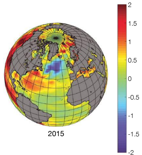
SST anomalies North Atlantic Ocean 2015
