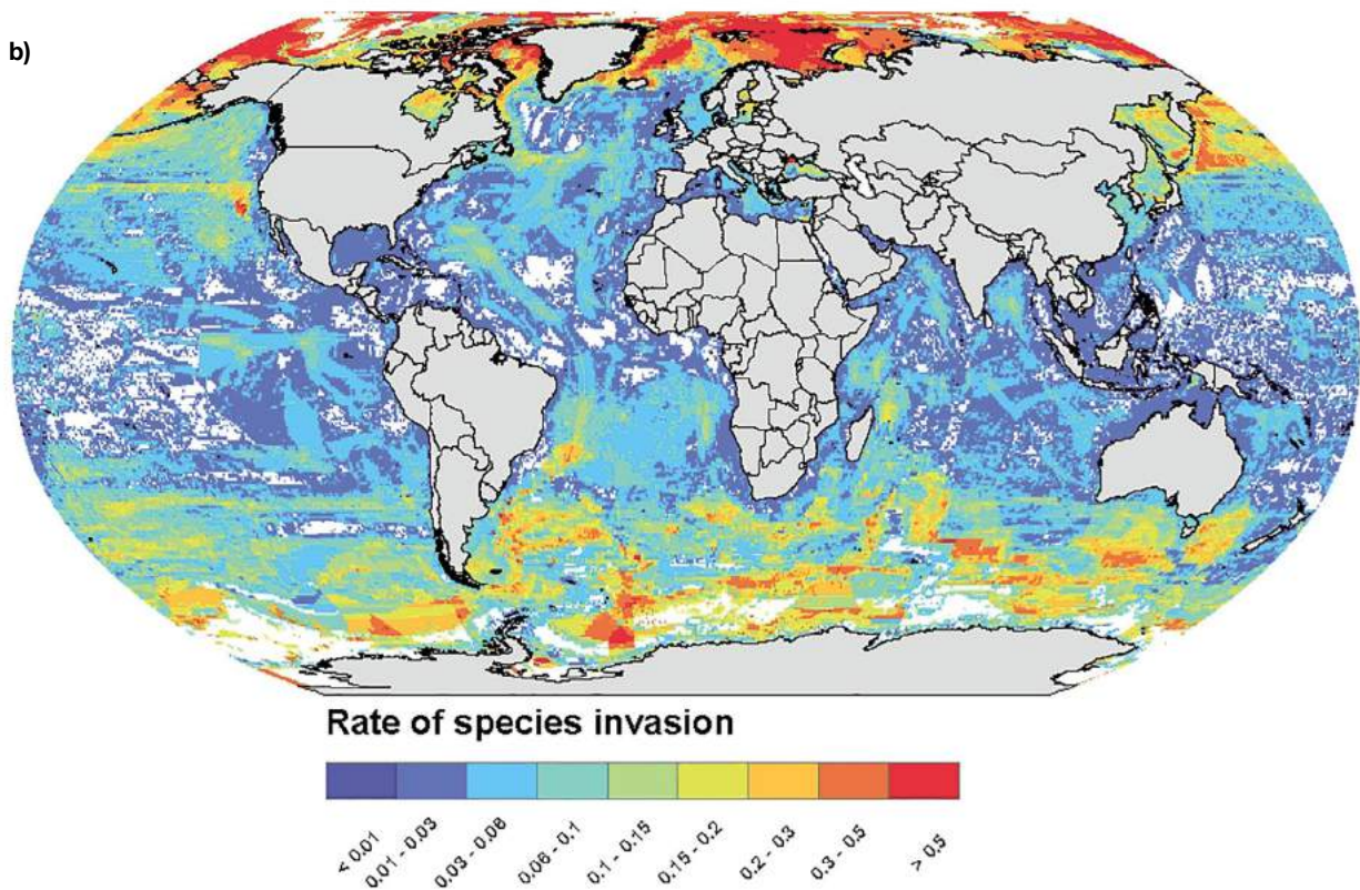
Figure 3.11.8 Projected intensity of (a) local extinction and (b) species invasion between 2000 and 2050 under the RCP 8.5 scenario (from Jones and Cheung, 2015). The unit is expressed as number of species locally extinct or invaded relative to the original species richness.
