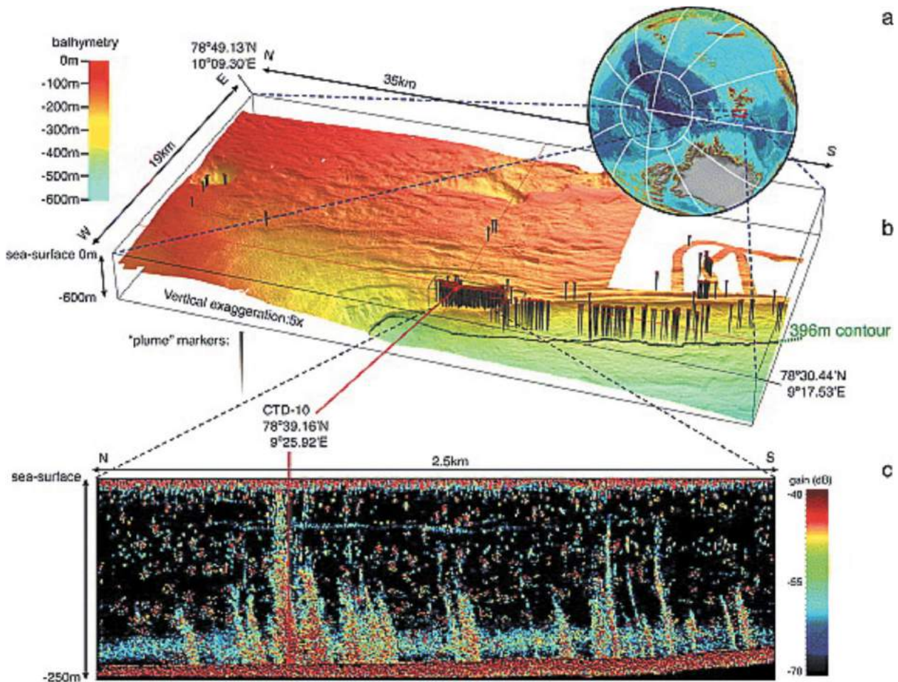
Figure 4.2.4 from Westbrook et al. (2009). (a) Location of survey area west of Svalbard; IBCAO bathymetry (Jakobsson et al. , 2008). (b) Positions of plumes acoustically imaged with the EK60 sonar, depicted by “pins”, superimposed on perspective view of the bathymetry of part of the area of plume occurrence. Bathymetry is from EM120 multibeam survey of cruise JR211 gridded at 20-m resolution, combined with high-resolution survey data from the Norwegian Hydrographic Service for the shallower-than-200-m part of the map. The 396-m isobath is the expected landward limit of the GHSZ. (c) Part of record from an EK60 acoustic survey from JR211, showing examples of observed plumes. Amplitude of acoustic response is given by the colour of the “bubbles”. All plumes show a deflection towards the north caused by the West Svalbard Current. The sea bed, at around 240-m depth, is shown by the strong (red) response. The position of CTD cast 10 is indicated by vertical red arrow.
