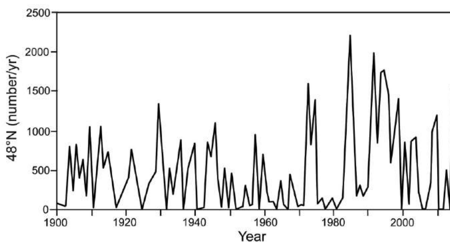
Figure 4.1.5 Total number of icebergs >5 m in diameter crossing latitude 48°N in the NW Atlantic each year 1900–2014, as recorded by the IIP. Note that the year is defined as an ice-year, beginning in October of the year before the notional record and extending to September of the ordinal year. Reproduced from Bigg (2016), with permission of Cambridge University Press.
