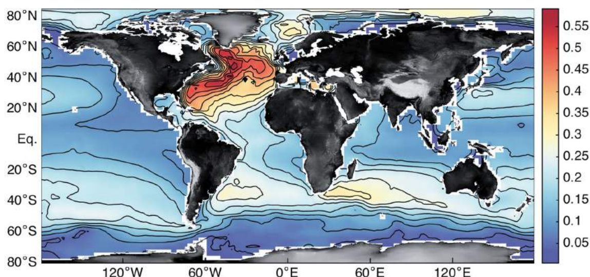
Figure 4.2.2 Estimated accumulation of anthropogenic carbon in the water column. Contours are every 0.043 \text{ mol m}^{-2} \text{yr}^{-1} . Adapted from control run of ocean assimilation model of DeVries (2014).
