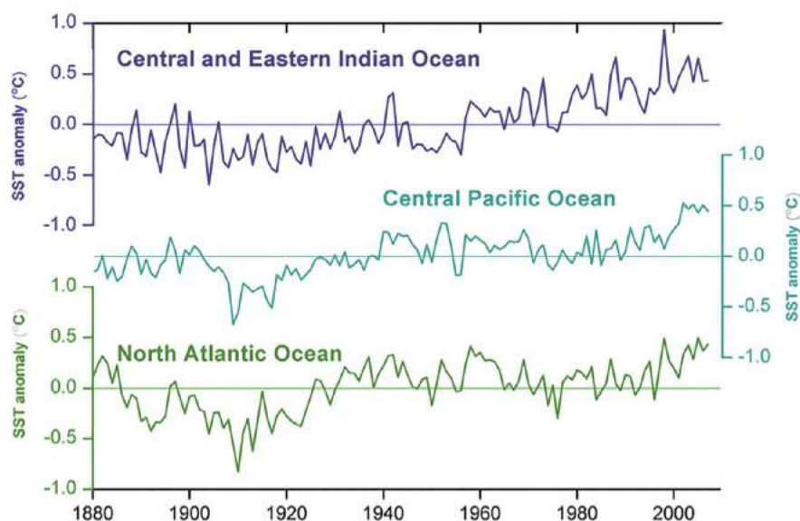
Figure 3.8.3 Sea-surface temperature (SST) time-series for reef-containing locations within three regions showing trend of increasing temperatures through the period 1880–2007. After Heron et al. (2009).
