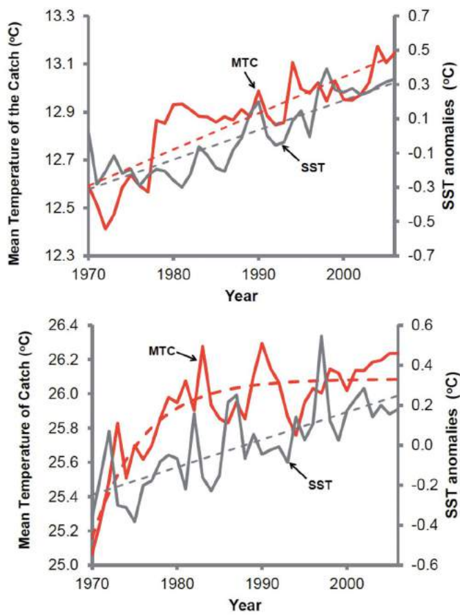
Figure 3.11.7 Average mean temperature of catch (MTC) and sea surface temperature (SST) from (upper) non-tropical and (lower) tropical large marine ecosystems (left panels). The right panels are schematic representation of hypotheses explaining the change in MTC over time (from Cheung et al. , 2013a).
