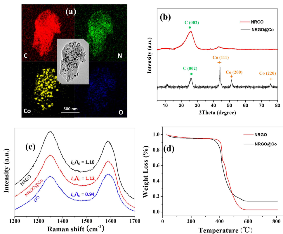
Figure 3. Elemental mapping of NNRGO@Co (a) XRD spectra (b), Raman spectra (c), and TGA spectra (d) of NRGO and NRGO@Co samples.
