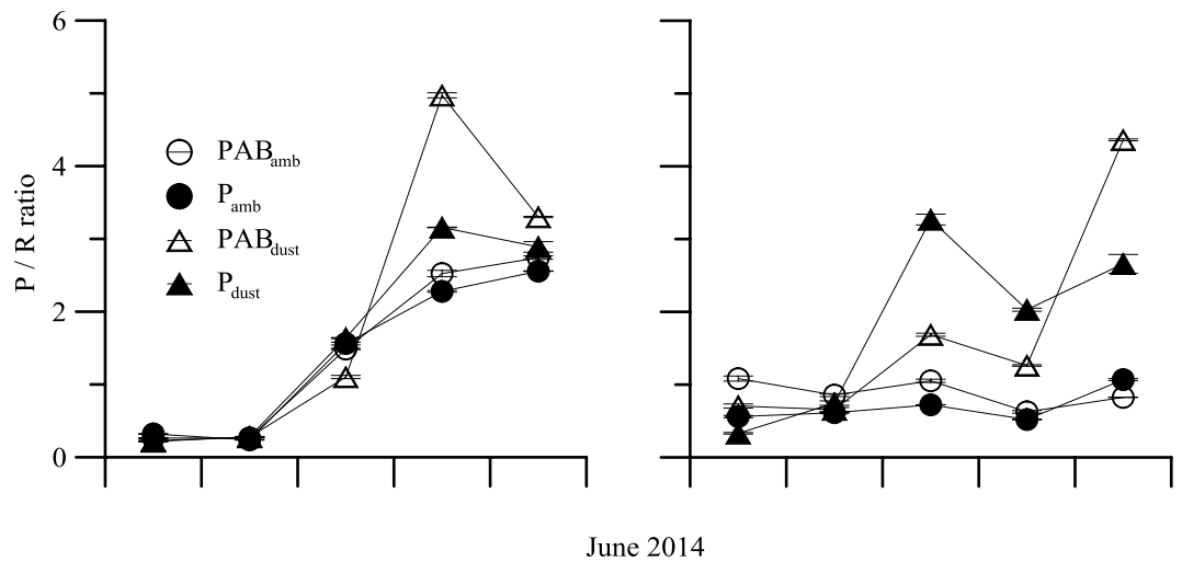
Figure 5. Mean ( \pm SD) total production/respiration (P/R) ratios ( A,B ) under two radiation treatments, PAB ( >280 nm) and PAR ( P > 400 nm) and two nutrient treatments, ambient (amb) and dust during the experiments in the heterotrophic and autotrophic area.
