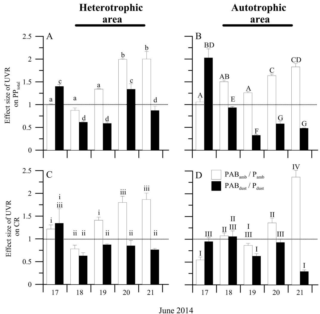
Figure 4. Effect size of UVR (as PAB/PAR ratio) on the mean ( \pm SD) total primary production ( A,B ) ( PP_{total} , in mmol\ C\ m^{-3}\ d^{-1} ) and ( C,D ) mean ( \pm SD) community respiration (CR) rates (in mmol\ C\ m^{-3}\ d^{-1} ) in the microcosms during the experiment under two dust treatments, ambient (amb) and dust, in the heterotrophic and autotrophic area. The letters on top of the bars indicate the result of the LSD post hoc test, and the horizontal dashed line delineates the positive ( >1 ) or negative ( <1 ) ultraviolet radiation effects.
