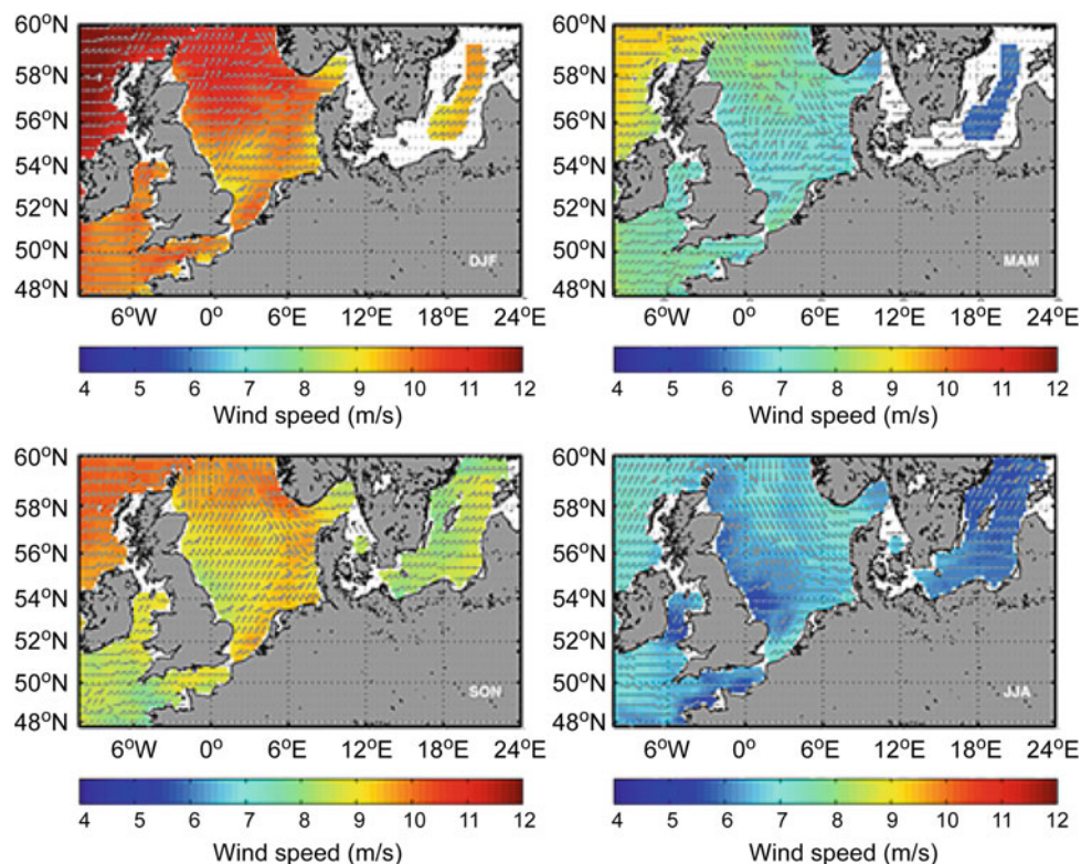
Fig. 1.20 Spatial distribution of seasonal mean wind speed ( \text{m s}^{-1} ) and the most frequently observed wind direction ( arrows ) derived from QuikSCAT satellite data for the period November 1999 to October 2009 (Karagali et al. 2014)
