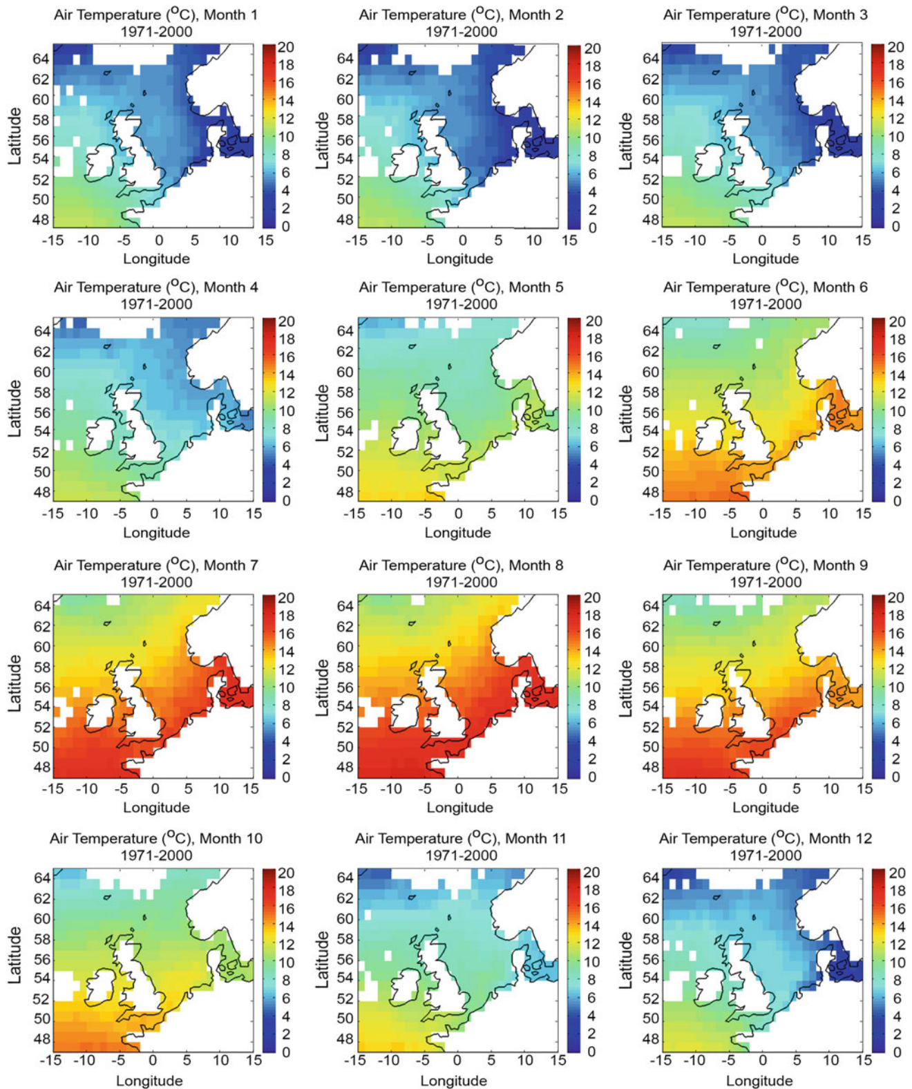
Fig. 1.25 Spatial distribution of monthly mean air temperature (°C) across the North Sea region based on in situ data for the period 1971–2000 (Stammer et al. 2014)
