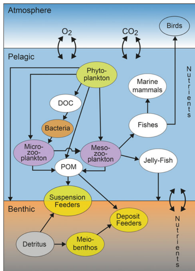
Fig. 1.34 Schematic overview of the trophic structure and flows of energy in the North Sea
