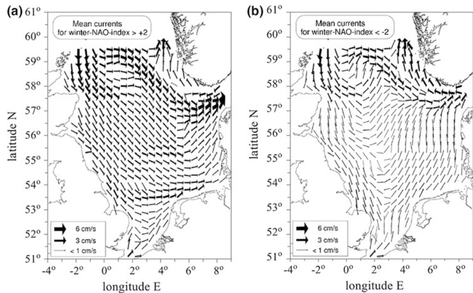
Fig. 1.12 North Sea circulation during prevailing positive winter NAO conditions ( left ) and negative winter NAO conditions ( right ) (Schrum and Siegmund 2001)
