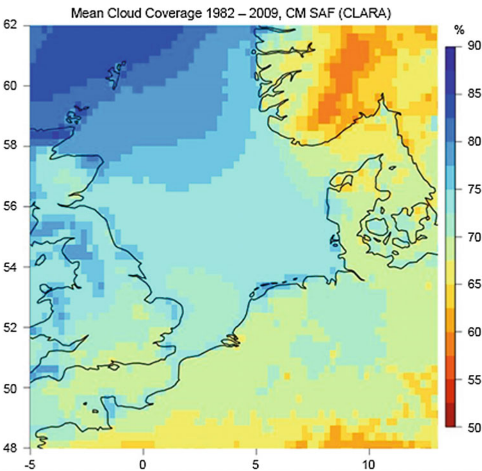
Fig. 1.32 Mean annual cloud coverage (in percentage) for the period 1982–2009 derived from satellite data by CM-SAF
