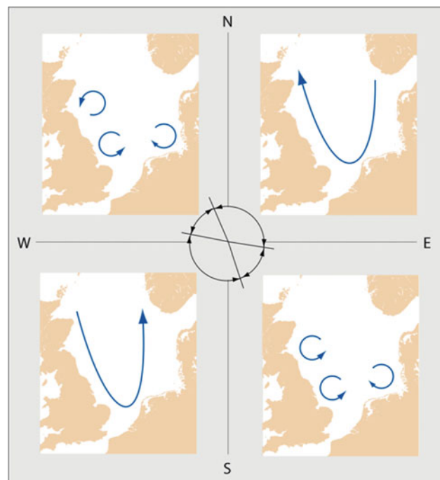
Fig. 1.11 Basic wind-driven circulation patterns in the North Sea. The four current states correspond to the four wind direction sectors in the central diagram (after Sündermann and Pohlmann 2011)
