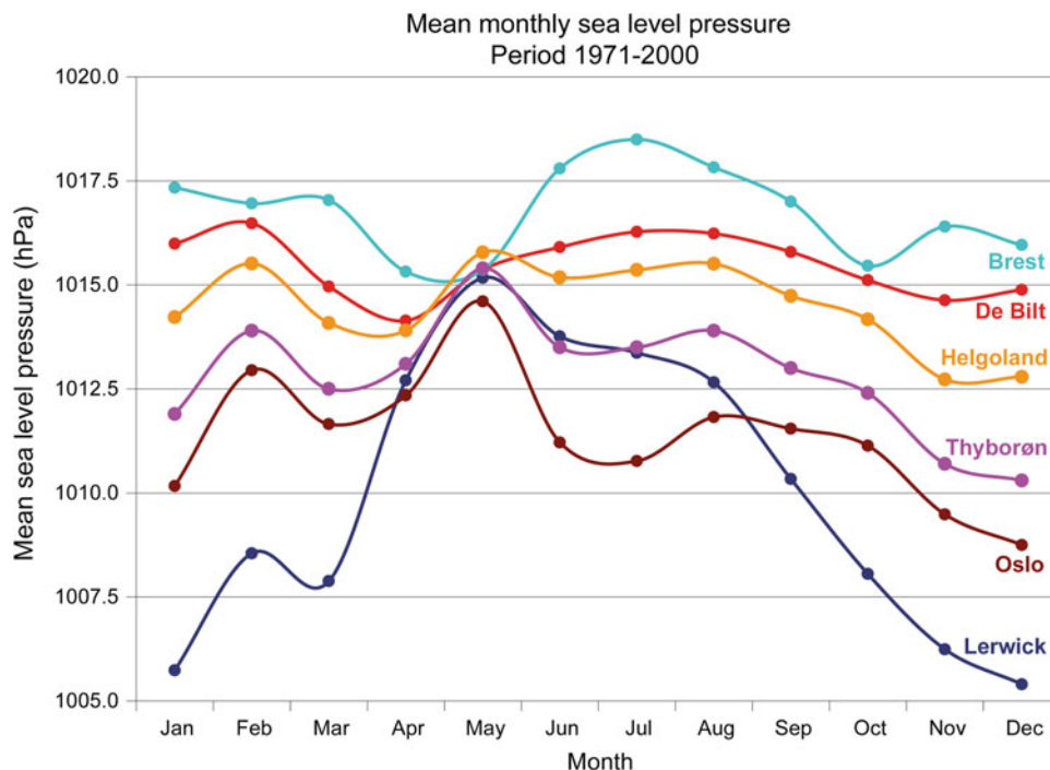
Fig. 1.18 Annual cycle of mean sea-level pressure (hPa) at selected land stations in the North Sea region for the period 1971–2000. Station positions are shown in the E-Supplement to this chapter (Fig. S1.5.1)
