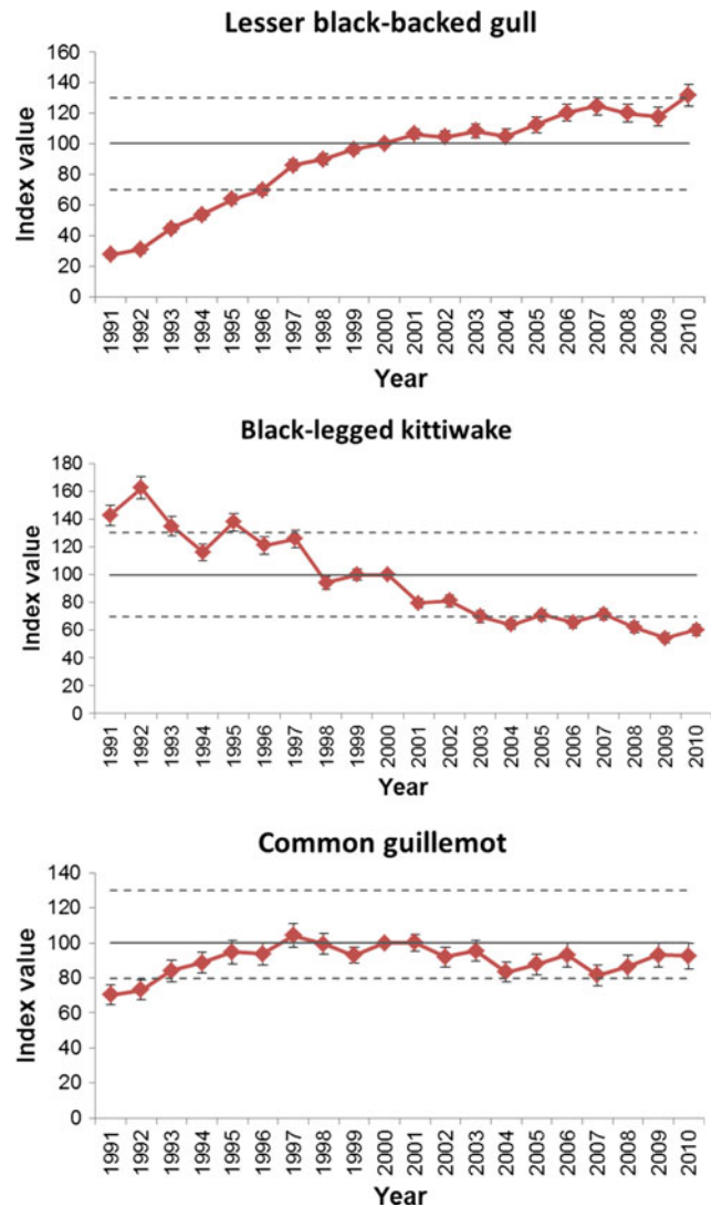
Fig. 8.10 Contrasting population trends for three seabird species breeding in the Greater North Sea from 1991–2010 (OSPAR Region II). Year 2000 was chosen as the baseline with the index value set to 100. Vertical lines show standard errors. ICES (2011)
