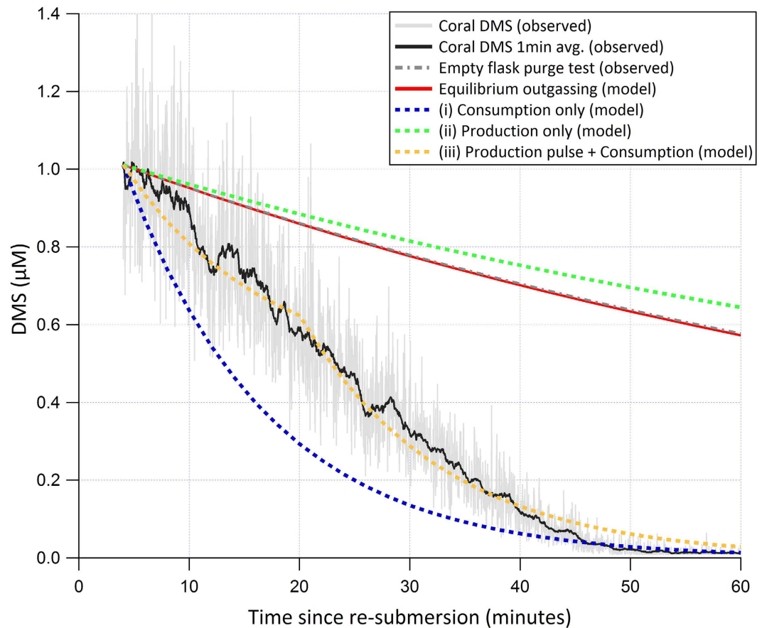
Figure 4. Observations and model results for \text{DMS}_{\text{sw}} in an experimental flask holding an Acropora cf. horrida colony. API-CIMS measurements (black line: 1 min average) commenced upon coral re-submersion following 16 min of exposure to air (Stage III). Grey dashed line represents the exponential loss of DMS due to bubbling based on measurements made in a coral-free flask derived during a separate experiment. The red line shows the calculated loss rate due to equilibrium outgassing. Results of model runs: (i) loss rate in absence of DMS production with a first order consumption rate of 3.7/hr (blue dashed line); (ii) zero consumption and a constant production rate of 100 nM/h (green dashed line); (iii) first order consumption rate of 3.7/hr and high production of 2 \mu\text{M}/\text{h} for first 15 min followed by zero production (gold dashed line).
