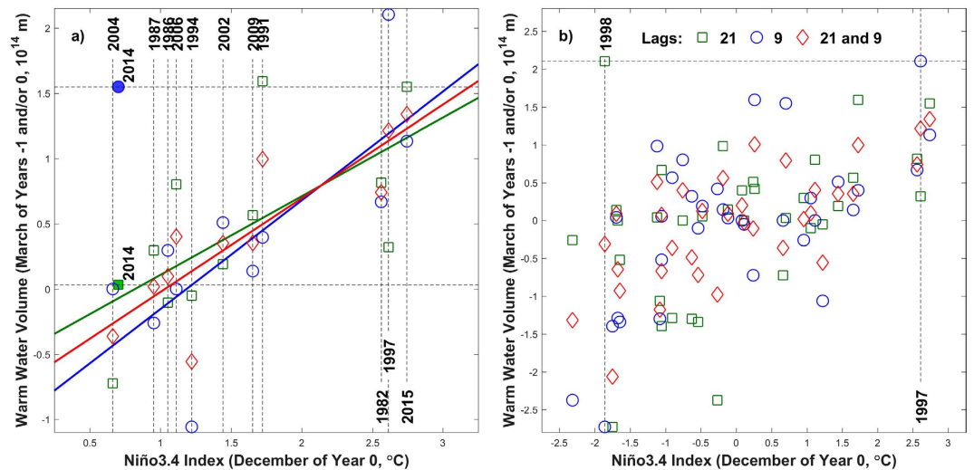
Figure 1. Observed relationship between the December anomaly of the Niño3.4 Index (in ^{\circ} C) and leading Warm Water Volume anomalies ( 10^{14} m) in March of the same year (blue circles), March of the preceding year (green squares), and the average of both years (red diamonds). Episodes in panel a correspond to all El Niño events since 1980 according to the NOAA's Climate Prediction Center (vertical dashed lines, 33), with colored straight lines depicting the linear fitting, while panel b shows values for all years in the 1980–2015 period. The 21-month (9-month) lag relationship corresponding to the neutral year of 2014 is additionally shown as a solid square (circle) in panel a. Warm Water Volume was computed as the volume of water masses above the 20^{\circ} C isotherm within 120E–80W and 5S–5N.
