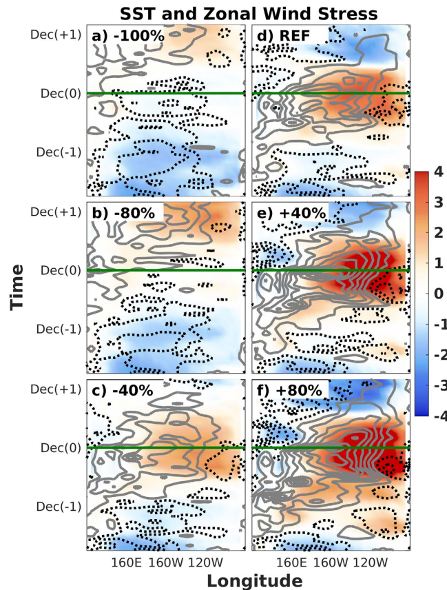
Figure 3. Longitude-time Hovmöller diagram of sea surface temperature (shading, in °C) and zonal wind stress (contour, in N/m 2 ) anomalies. Panels correspond to the −100% (a), −80% (b), −40% (c), REF (d), +40% (e) and +80% (f) experiments. The minimum contour is \pm 0.005 N/m 2 and the contour interval is 0.01 N/m 2 , with grey solid (black dashed) lines depicting positive (negative) anomalies. The horizontal green lines indicate the December month in which El Niño peaks in the reference simulation.
