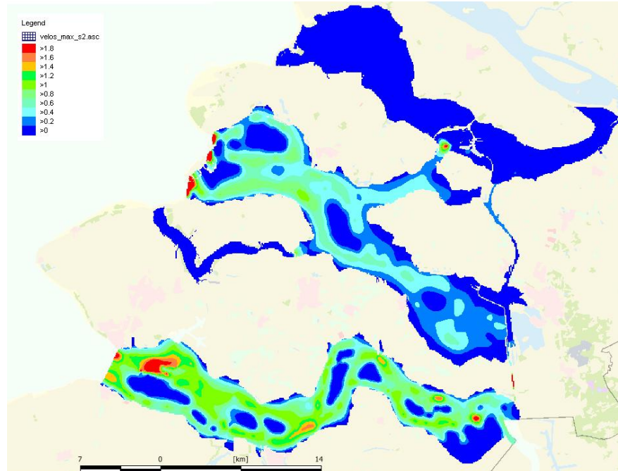
Figure 3.11: flow velocity(m/s) for scenario 1 (maximum over 1 year).
