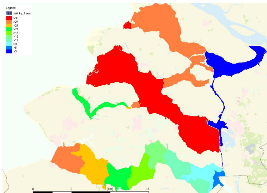
Figure 3.1: Salinity (ppt) for the baseline scenario (average over 1year).
