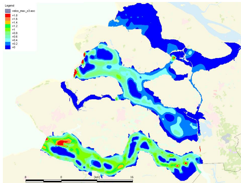
Figure 3.12: flow velocity (m/s) for scenario 2 (maximum over 1 year)
