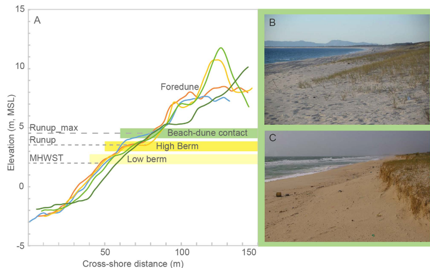
Figure 2. Examples of modern beach profiles extracted from the LiDAR dataset pointing out the location of the indicators used to track sea-level rise: the berm (high berm) and the contact between the dune and the beach (A). Note the presence of a second lower berm consequence of changes in wave climate and tidal cycles 55 . Pictures show the contact between the beach and the dune characterized by incipient vegetated dunes (B) and dune scarp (C). Mean high water during spring tides (MHWST), theoretical modal runup values calculated for non-storm conditions (Runup), and maximum runup values measured in situ following a major storm event (Runup_max).
