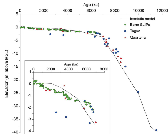
Figure 5. Plot comparing our data (berm indicators), the SLIPs from the Tagus estuary 66 , Quarteira 34 and the isostatic model proposed by Leorri et al. 29 for the Tagus estuary. The smaller panel shows the zoom into the time interval of focus of our study.
