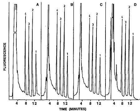
FIG. 1. Chromatograms obtained on extracts of turbot larvae supplemented with α-, γ-, and δ-tocopherol and tocol using different extraction methods. A, monophasic extraction with methanol; B, homogenization in hexane-methanol; C, double-phase extraction with hexane before the addition of water; D, saponification + double-phase extraction. Chromatographic conditions, see text. Peak identification: 1, α-tocopherol; 2, γ-tocopherol; 3, δ-tocopherol; 4, tocol (internal standard).
