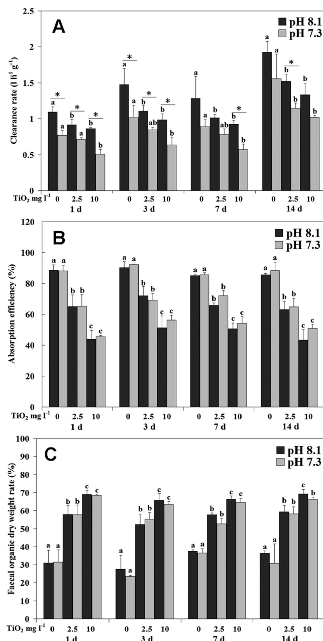
Figure 1. Clearance rate (CR, A ), Absorption efficiency (AE, B ) and faecal organic weight rate (E, C ) of M. coruscus exposed to six treatments for 14 days. The values with different superscripts at each pH are significantly different among three nano-TiO 2 treatments ( P < 0.05 ). The values denoted by an asterisk between two pH groups at each nano-TiO 2 concentration are significantly different ( P < 0.05 ).
