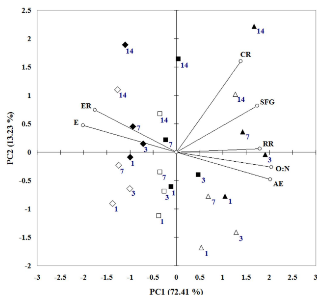
Figure 4. Principal component analysis (PCA) by integrating all measured parameters (CR, AE, RR, ER, O:N, SFG, E) for four times (days: 1, 3, 7 and 14) and six different treatments (▲-TiO 2 0 × pH 8.1, △-TiO 2 0 × pH 7.3, ■-TiO 2 2.5 × pH 8.1, □-TiO 2 2.5 × pH 7.3, ◆-TiO 2 10 × pH 8.1, ◇-TiO 2 10 × pH 7.3) with a biplot. Both the scores of the experimental conditions and the loadings of the parameters (O) were present.
