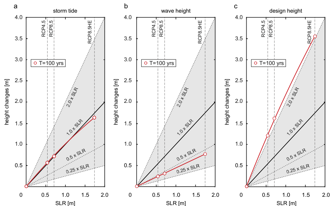
Figure 4. Relationship between different SLR projections and storm tides, waves, and design heights at western Pellworm. For all RCP based SLR projections the feedback in the ARI_{100} (red lines) of (a) storm tides; (b) wave heights; and, (c) design heights is shown. Dashed lines mark changes compared to SLR covering scaling factors equal to 0.25, 0.5, 1.0 and 2.0.
