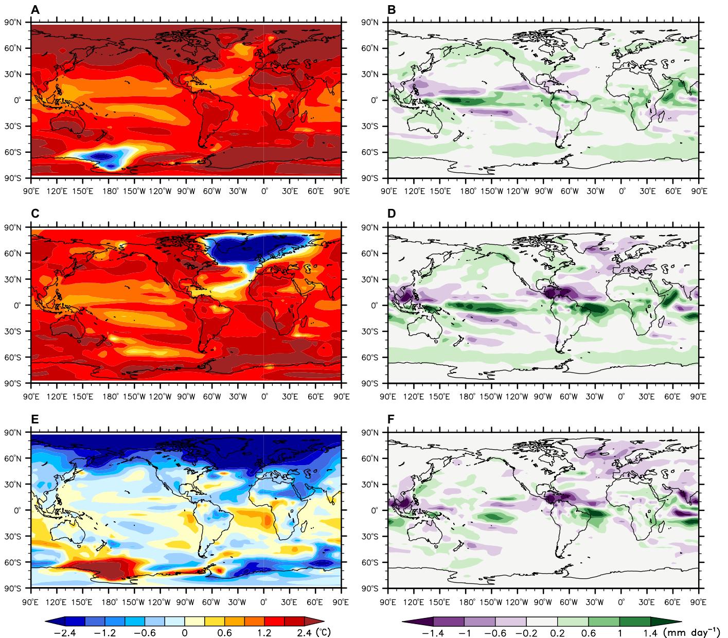
Fig. 4. Long-term (after 300 years) responses of surface temperature and precipitation to CO 2 increase. (A, C, and E) Results of annual mean temperature (shading in °C): (A) the CTLCO 2 minus the CTL (C) the ADJCO 2 minus the ADJ, and (E) the difference between (C) and (A). (B, D, and F) Similar to (A), (C), and (E) but for the results of annual mean precipitation (shading in mm day -1 ).
